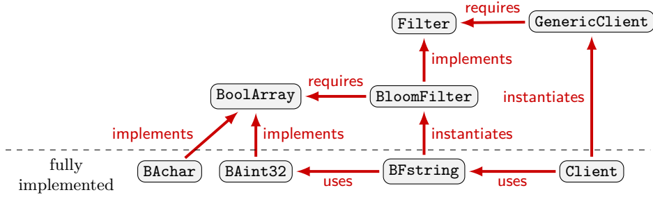
Fig. 2. Bloom filters in Why3: the module map.
