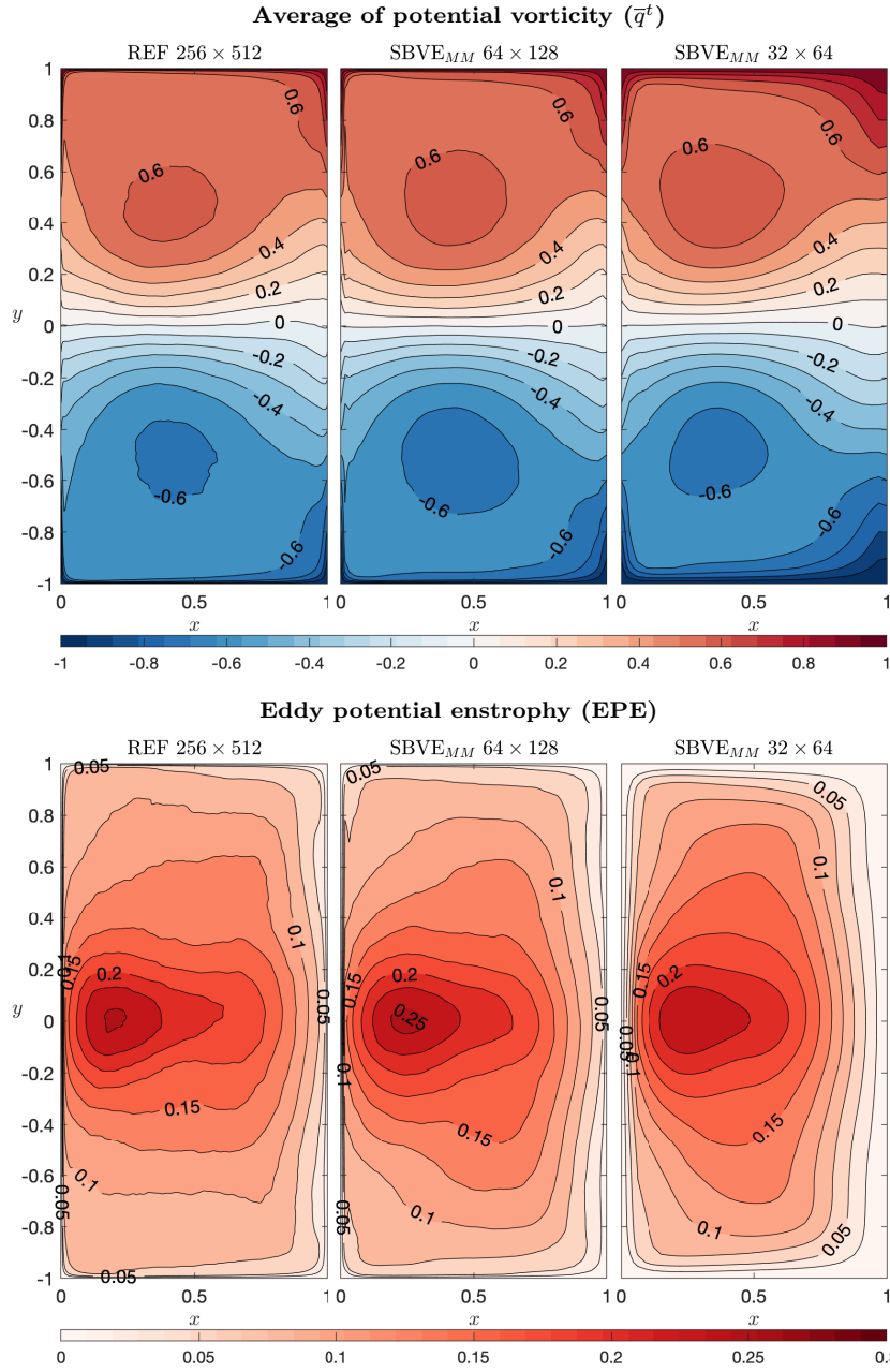
Figure 12: Contour plots showing the qualitative convergence of the statistics for \text{SBVE}_{\text{MM}} . The top three plots describe the averaged PV with CI of 0.1, and the bottom three show EPE with CI of 0.025. In each panel, the first one stands for BVE 256 \times 512 , the second one is \text{SBVE}_{\text{MM}} 64 \times 128 and the third one is \text{SBVE}_{\text{MM}} 32 \times 64 .
