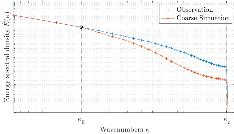
Figure 2: Illustration of the time-averaged kinetic energy spectrums. The wavenumber \kappa_0 is searched as the first point where the observation and the coarse-simulation BVE deviate, in order to estimate \gamma_0 from (4.3c).
