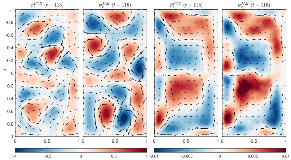
Figure 6: Instantaneous snapshots of the small-scale random stream functions \psi_r^{\text{POD}} , \psi_r^{\text{MM}} and the Itô–Stokes stream functions \psi_s^{\text{POD}} , \psi_s^{\text{MM}} , resp. provided by the \text{SBVE}_{\text{POD}} and the \text{SBVE}_{\text{MM}} at resolution 64 \times 128 . The associated small-scale random velocity \frac{1}{\Delta t} \sigma d\mathbf{B}_t is indicated here by the black arrows. Note that these velocity fields are located on the \psi -grid (see 15) through linear interpolations.
