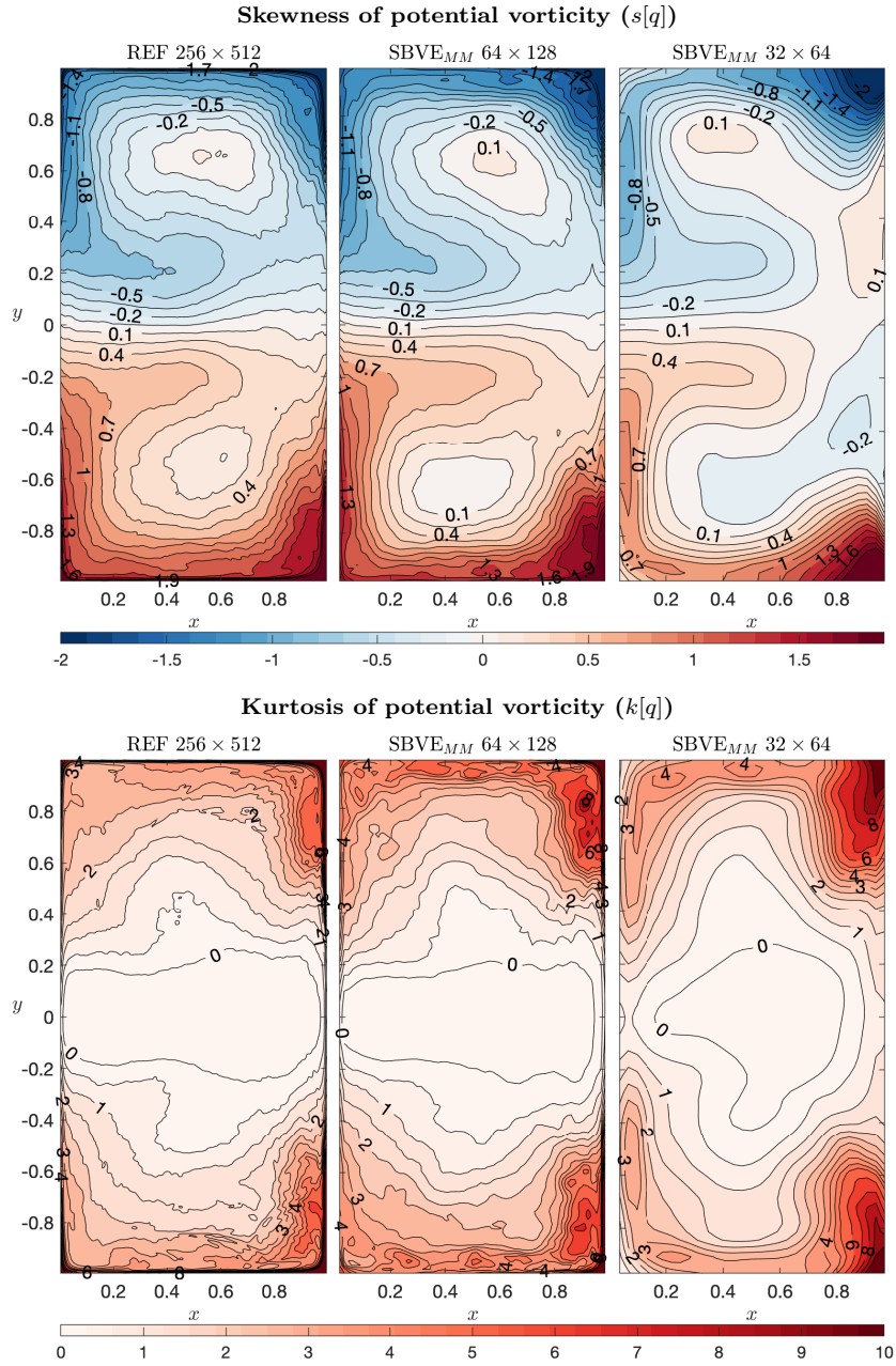
Figure 13: Contour plots showing the qualitative convergence of the statistics for SBVEMM. The top three plots depict the PV-skewness with CI of 0.15, and the bottom three show the PV-kurtosis with CI of 0.5 within [0, 4.5] and of 1 within [5, 10] . In each panel, the first one is BVE 256 \times 512 , the second one is SBVEMM 64 \times 128 and the third one is SBVEMM 32 \times 64 . The visualized quantity is not defined on the boundary of both fields.
