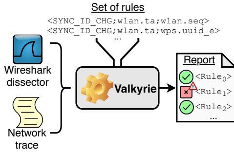
Figure 2: Functional diagram of Valkyrie . A network trace along with a set of rules are provided as inputs to the tool. The Wireshark dissector is leveraged for the protocol field denomination that must be specified in rules. At the end of the analysis, Valkyrie outputs a report specifying verified rules and breached ones with detailed warning messages.
