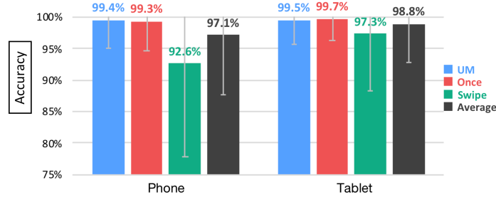
Fig. 7. Accuracy performance for individual input method on both phone and tablet for the two-handed conditions. Error bars show 95% confidence intervals. Ordinate axis starts at 75%
