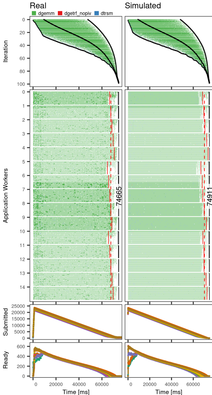
Fig. 5: The 3×5 BC partitioning using 15 identical CPU-only nodes to compare the behavior of a real execution (left) against the simulation (right): the simulation captures the load imbalance coming from the BC distribution.
