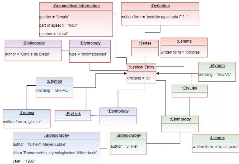
Figure 7: The LMF encoding for cócoras .
