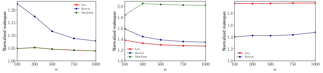
Figure 5: Performance for roofline model (left), communication model (middle) and Amdahl's model (right) with P = 7500 , \lambda = 10^{-7} and n \in [100, 1000] .
