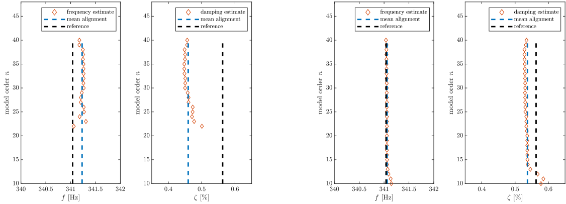
Figure 14: Modal alignments of the natural frequency and damping ratio estimates for the first structural mode from measurements before (left) and after (right) the removal of the periodic subsignal.
