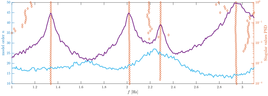
Figure 18: Stabilization diagram of the natural frequency estimates from measurements of the ship after the removal of the periodic subsignal.
