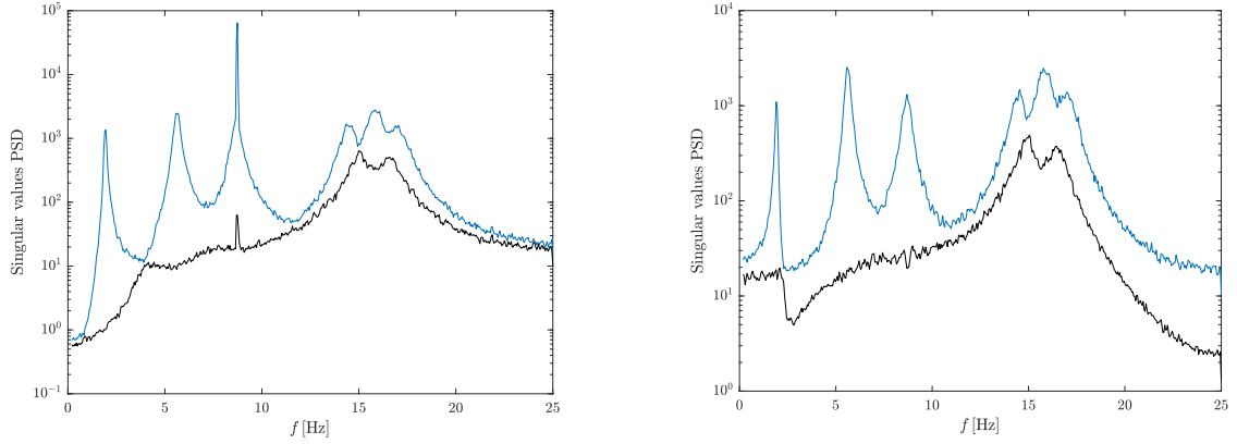
Figure 8: Two largest singular values of PSD matrix from raw data y_k (left) and from projected data \hat{y}_k^{\text{pro}} after removal of the periodic subsignal (right).
