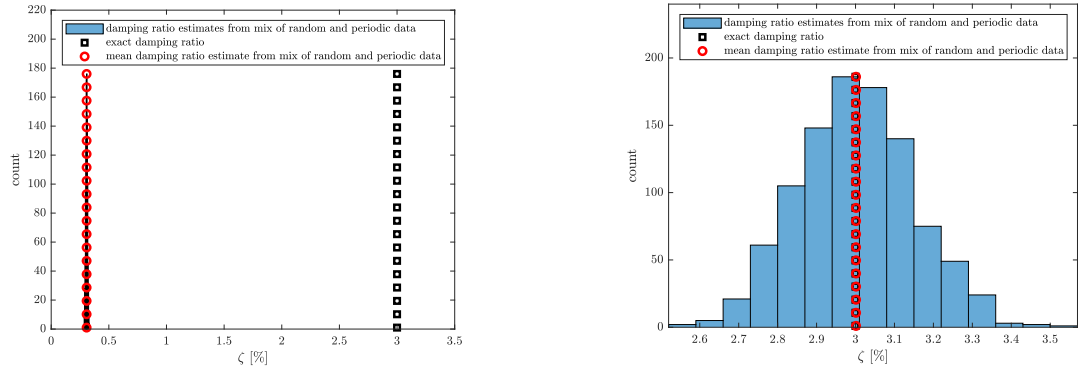
Figure 5: Histograms of the damping ratio of the third mode identified with model order 12 (left) and 14 (right).
