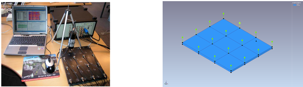
Figure 10: The experimental setup: plate with 16 acceleration channels, shaker, acquisition system (left). The plate model with 16 acceleration channels in ARTEMIS MODAL PRO 6.0 (right).
