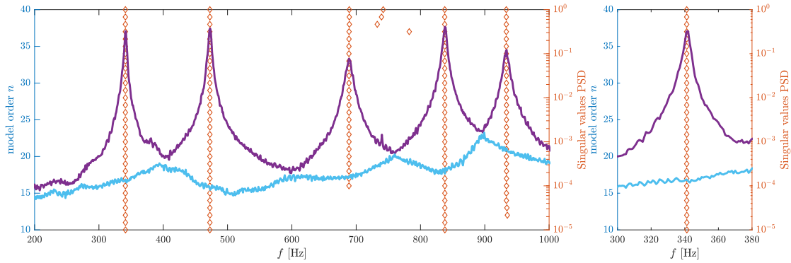
Figure 13: Stabilization diagram of the natural frequency estimates from measurements of the plate after the removal of the periodic subsignal.
