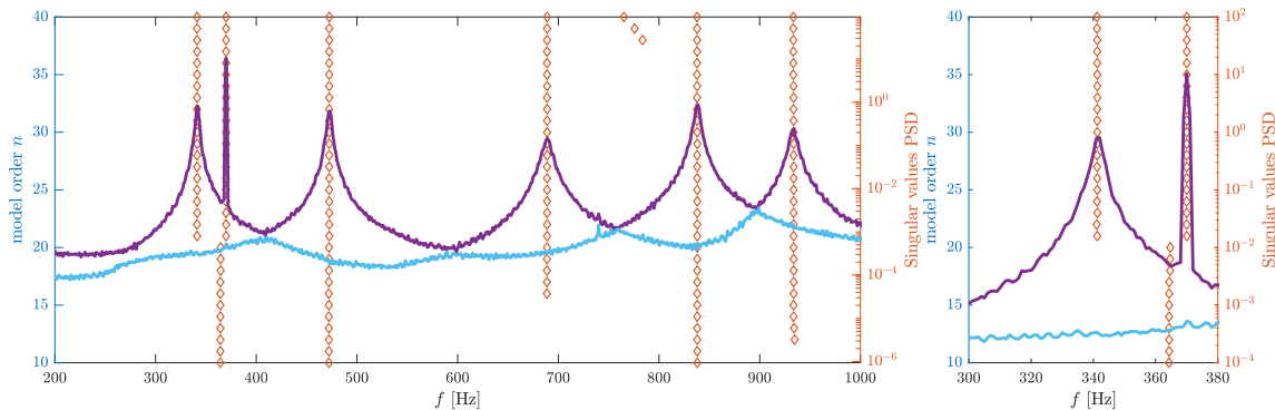
Figure 11: Stabilization diagram of the natural frequency estimates from the raw measurements of the plate containing both structural and periodic modes.
