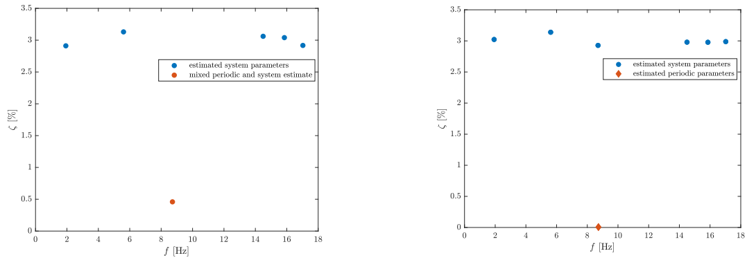
Figure 3: Estimates of natural frequency and damping ratio from one simulation. Model order 12 (left) and 14 (right).
