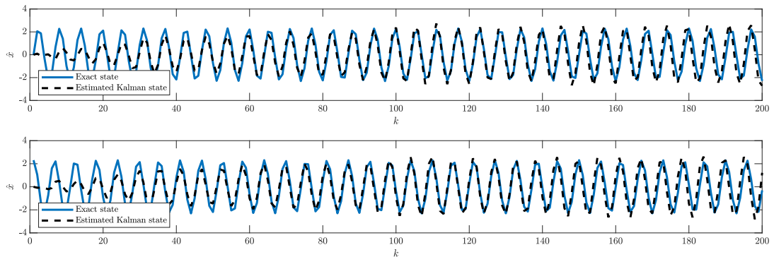
Figure 7: Exact states and computed Kalman states corresponding to the periodic mode.
