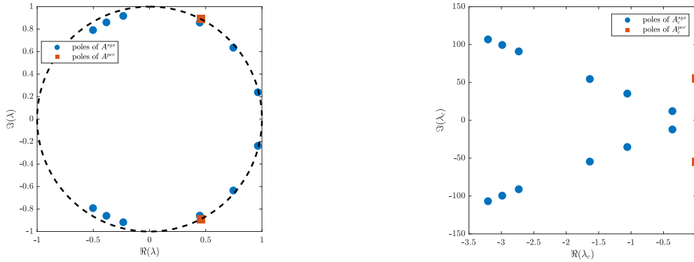
Figure 1: Discrete-time and continuous-time poles of the system from (12) and (14) respectively.
