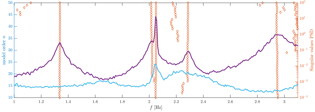
Figure 16: Stabilization diagram of the natural frequency estimates from the raw measurements of the ship containing both structural and periodic modes.
