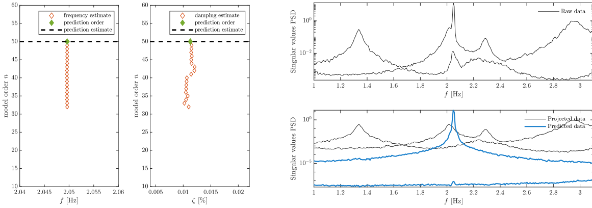
Figure 17: Left: Stable modal alignments of the natural frequency and damping ratio estimates of the periodic mode at 2.05 Hz. Right: Two largest singular values of PSD from raw measurements (top), and estimated periodic signal and projected data (bottom).
