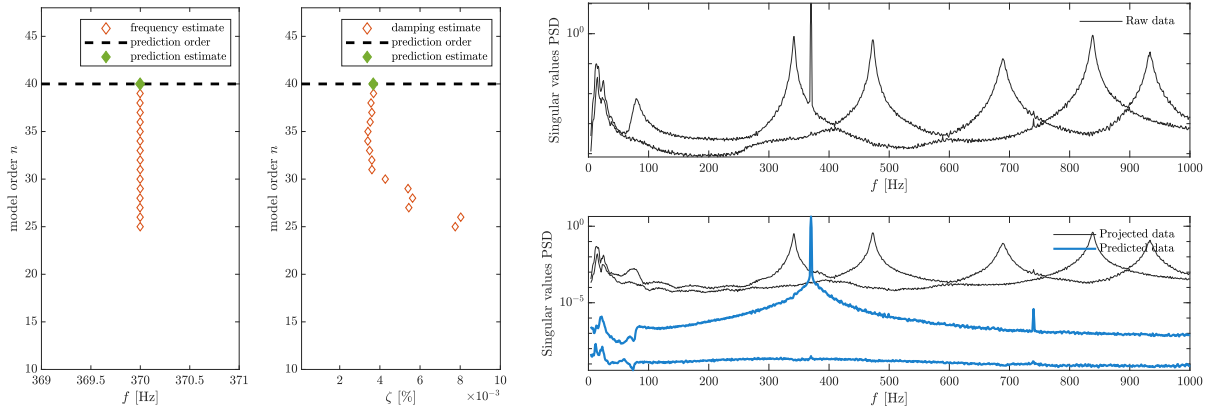
Figure 12: Left: Stable modal alignments of the natural frequency and damping ratio estimates of the periodic mode of the plate. Right: Two largest singular values of PSD from raw measurements (top), and estimated periodic signal and projected data (bottom).
