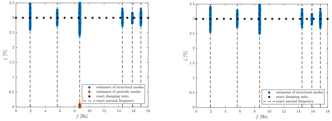
Figure 9: Estimates of natural frequencies and damping ratios from raw data y_k (left) and from projected data \hat{y}_k^{\text{pro}} after removal of the periodic subsignal (right) for the complete Monte Carlo simulation.
