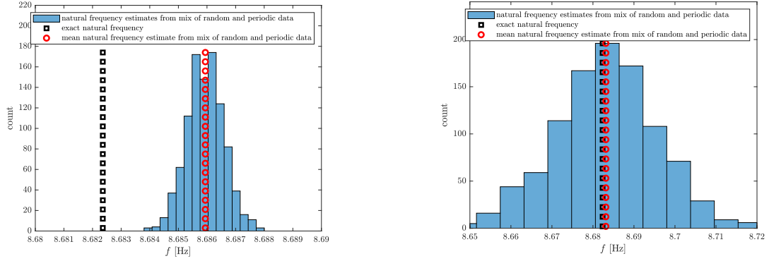
Figure 4: Histograms of the natural frequency of the third mode identified with model order 12 (left) and 14 (right).
