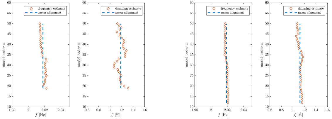
Figure 19: Modal alignments of the natural frequency and damping ratio estimates for the second structural mode (close to the periodic mode) from measurements before (left) and after (right) the removal of the periodic subsignal.
