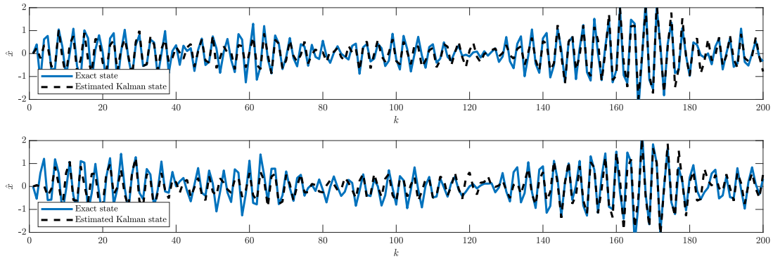
Figure 6: Exact states and computed Kalman states corresponding to the structural mode closest to the periodic mode.
