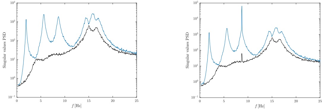
Figure 2: Two largest singular values of PSD matrix from output data of the system subjected to random (left) and mixed random and periodic (right) excitation.
