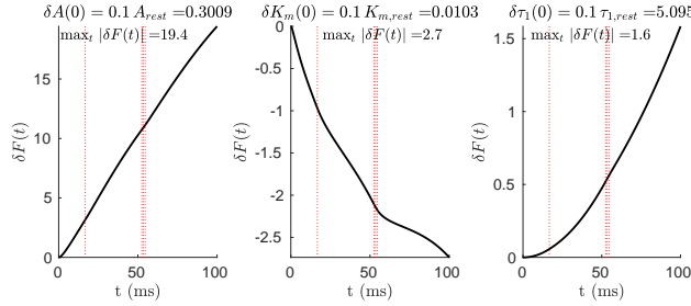
FIGURE 7. Sensitivity analysis. Time evolution of the Jacobi fields component \delta F(\cdot) where their initializations are 10% of the physical values A_{rest}, K_{m,rest}, \tau_{1,rest} associated to the trajectory of the force-fatigue model.
