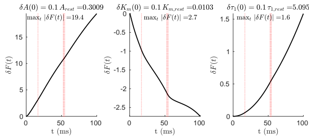
FIGURE 7. Sensitivity analysis. Time evolution of the Jacobi fields component \delta F(\cdot) where their initializations are 10% of the physical values A_{\text{rest}}, K_{m,\text{rest}}, \tau_{1,\text{rest}} associated to the trajectory of the force-fatigue model.
