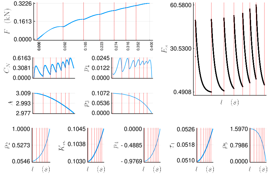
FIGURE 4. Time evolution on [0, T] , T = 0.4s of the state of the Ding et al model computed with the indirect approach maximizing \varphi(x(T)) = F(T) with n = 6 , I_m = 20ms . The optimal value is the same as the optimal value computed with the direct method (see Fig.3). The model parameters are given in Table 2.
