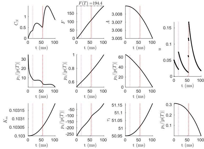
FIGURE 5. Extremal of the Ding et al model defined on [0, T] , T = 100ms , with four sampling times and maximizing the final force.
