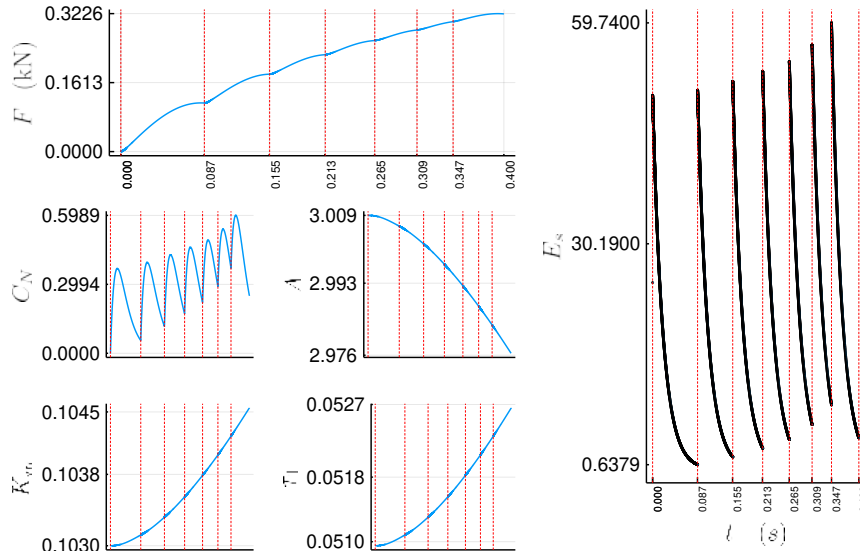
FIGURE 3. Time evolution on [0, T] , T = 0.4s of the normalized state of the Ding et al model computed with the direct approach maximizing \varphi(x(T)) = F(T) with n = 6 , I_m = 20ms . The model parameters are given in Table 2.
