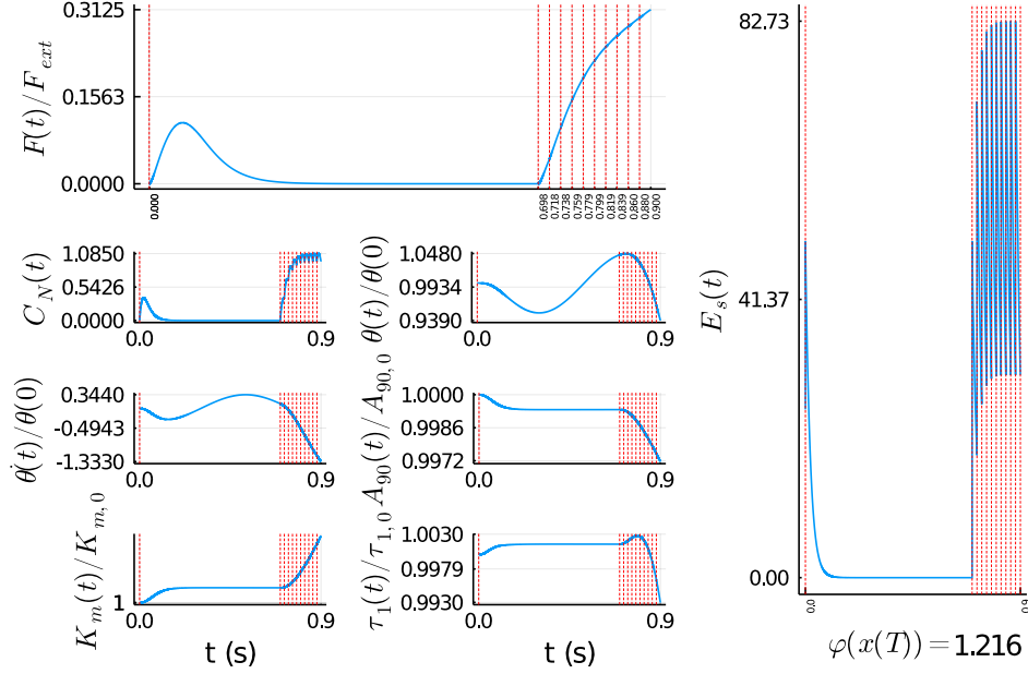
FIGURE 2. Time evolution on [0, T] , T = 0.9s of the normalized state of the Marion et al model when considering t_i = T - (n - i + 1)I_m , i = 1, \dots, n , n = 10 , I_m = 20ms . The model parameters are given in Table 1.
