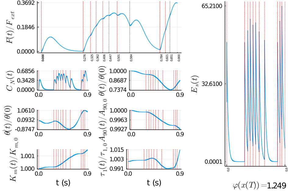
FIGURE 1. Time evolution on [0, T] , T = 0.9s of the normalized state of the Marion et al model computed with the direct approach maximizing \varphi(x(T)) = F(T)/F_{ext} + A_{90}(T)/A_{90,0} with n = 10 , I_m = 20ms . The model parameters are given in Table 1.
