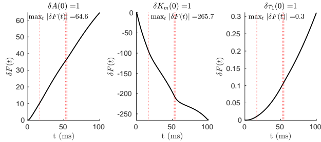
FIGURE 6. Sensitivity analysis. Time evolution of the Jacobi fields component \delta F(\cdot) according to Definition 2.7 and associated to the trajectory of the force-fatigue model.
