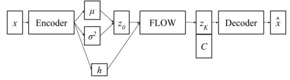
Figure 1: Inverse autoregressive flow model for acoustic model in parameteric expressive multispeaker TTS.
