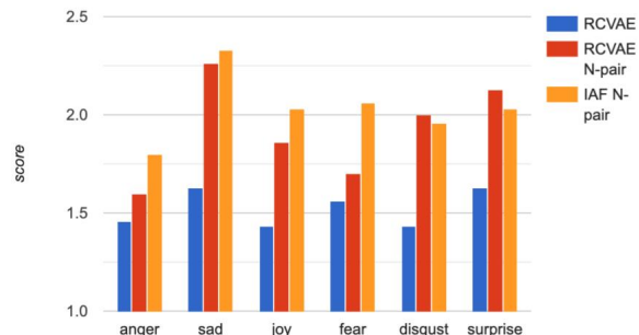
Figure 4: Expressive MOS score
