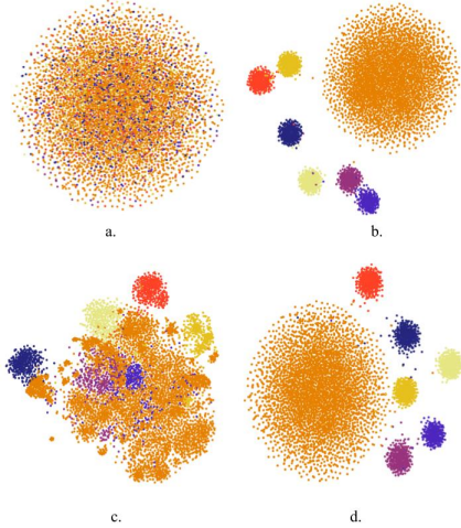
Figure 2: t -SNE plot of latent representation of IAF acoustic model (a.), IAF acoustic model with N -pair loss (b.), RCVAE acoustic model (c.), and RCVAE acoustic model with N -pair loss (d.); Each color in t -SNE plot represents emotion
