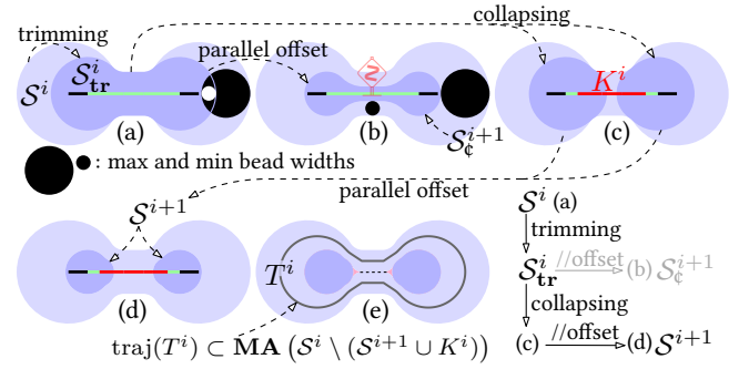
Fig. 4. The sequence of operations from S^i to S^{i+1} . (a) Trimming S^i . (b) A parallel offset of 2\gamma renders the dark blue shape S^{i+1}_tr less than 2\gamma -fat, which violates our required invariant. (c) Instead, we identify the narrow features of S^i by the set K^i of centers of medial-axis disks of radius smaller than 4\gamma . (d) S^{i+1} is obtained by removing K^i from the medial axis of S^{i+1}_tr and applying a 2\gamma -parallel offset. (e) The bead T^i is modeled between \partial S^i and \partial S^{i+1} \cup K^i . Its print trajectory is drawn in black. Gaps (pink pseudo-triangles) may remain between the bead T^i and S^{i+1} .
