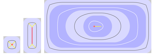
Fig. 11. Rectangles. 2\gamma = 0.3 mm, 2\Gamma = 1.0 mm. The rectangles have size 1x1, 2x1, 6x3 (in millimeters). The last state of the medial axis is shown.
