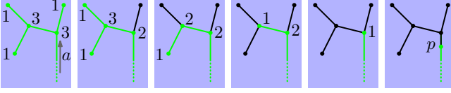
Fig. 7. Maximal trimmable w -trees are built from the leaves to the root. From left to right, each step processes one half-arc and a new set of a trimmable w -trees (black) is obtained. At the last step (right), a maximal trimmable w -tree \mathcal{T}_{p,a} is found. The number next to each vertex indicates its Normal -degree.
