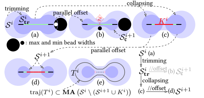
Fig. 4. The sequence of operations from \mathcal{S}^i to \mathcal{S}^{i+1} . (a) Trimming \mathcal{S}^i . (b) A parallel offset of 2\gamma renders the dark blue shape \mathcal{S}^{i+1}_c less than 2\gamma -fat, which violates our required invariant. (c) Instead, we identify the narrow features of \mathcal{S}^i by the set K^i of centers of medial-axis disks of radius smaller than 4\gamma . (d) \mathcal{S}^{i+1} is obtained by removing K^i from the medial axis of \mathcal{S}^i_{tr} and applying a 2\gamma -parallel offset. (e) The bead T^i is modeled between \partial\mathcal{S}^i and \partial\mathcal{S}^{i+1} \cup K^i . Its print trajectory is drawn in black. Gaps (pink pseudo-triangles) may remain between the bead T^i and \mathcal{S}^{i+1} .
