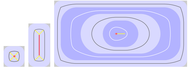
Fig. 11. Rectangles. 2y = 0.3 mm, 2\Gamma = 1.0 mm. The rectangles have size 1x1, 2x1, 6x3 (in millimeters). The last state of the medial axis is shown.
