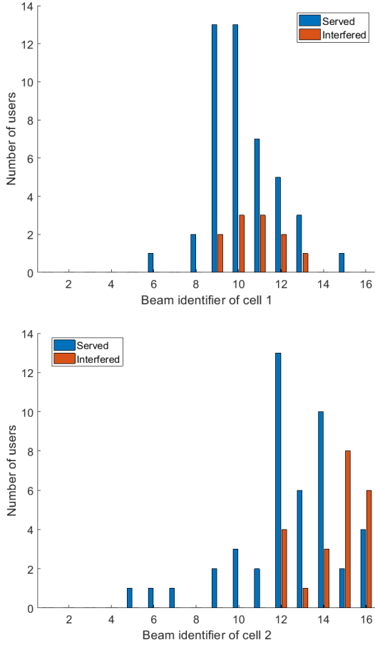
Fig. 5: Number of served and interfered users per beam
