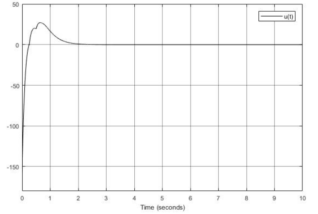
Fig. 5. Control law u_c(t)
