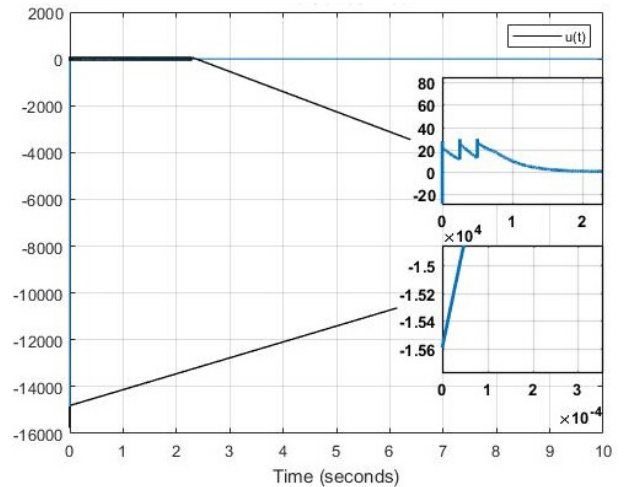
Fig. 1. Control law (44) with N = -5, k = 0.1 and r = 0.00072
