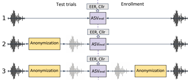
Figure 1: ASV evaluation.
