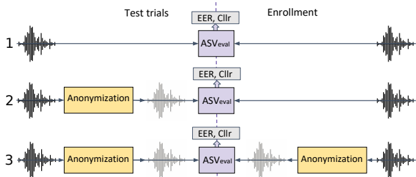
Figure 1: ASV evaluation.
