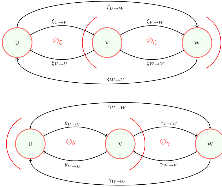
Fig. 2 Proof of associativity
