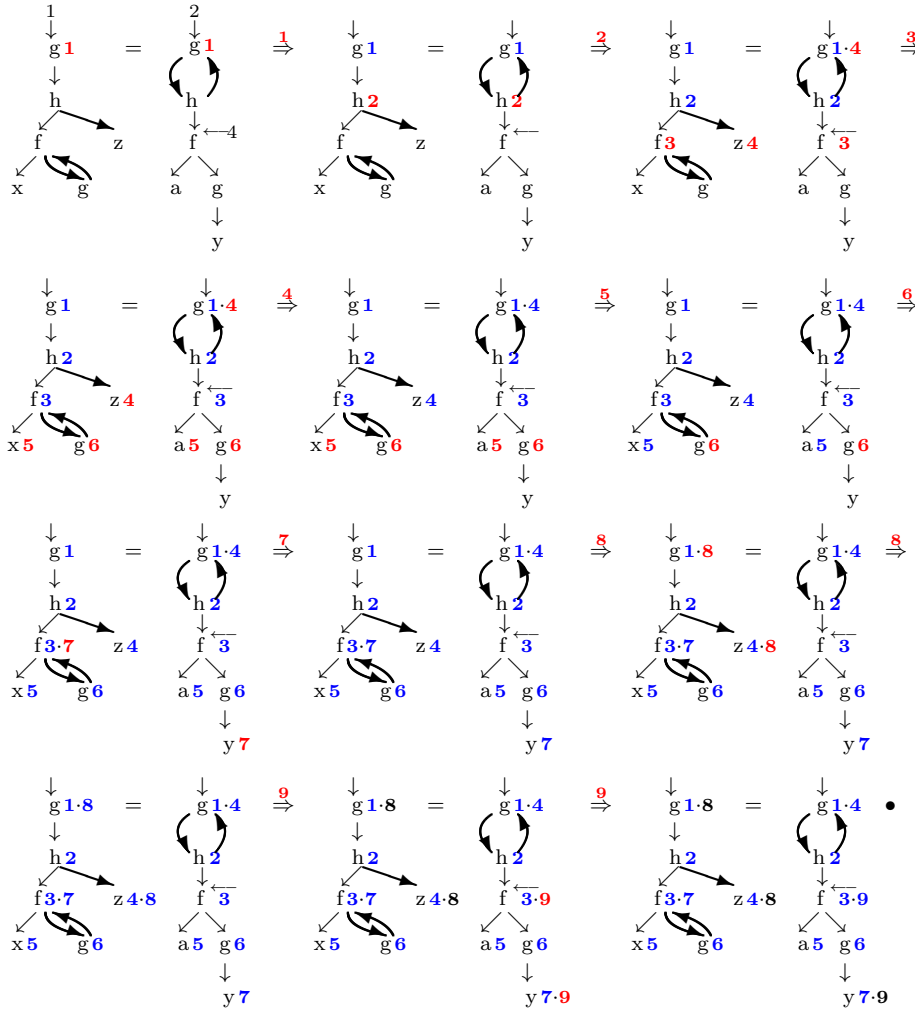
Fig. 9 Successful unification of two patterns.
