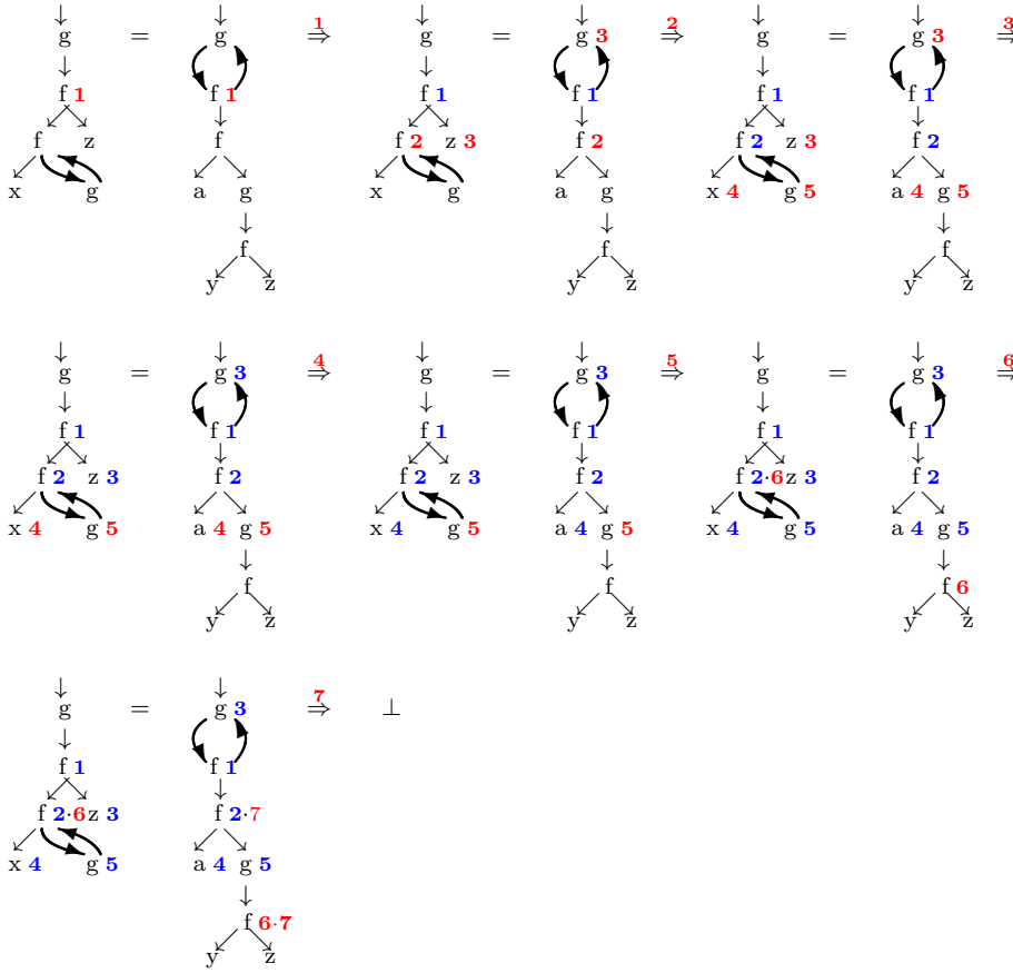
Fig. 10 Unification of two patterns (failure case).
