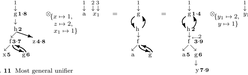
Fig. 11 Most general unifier
