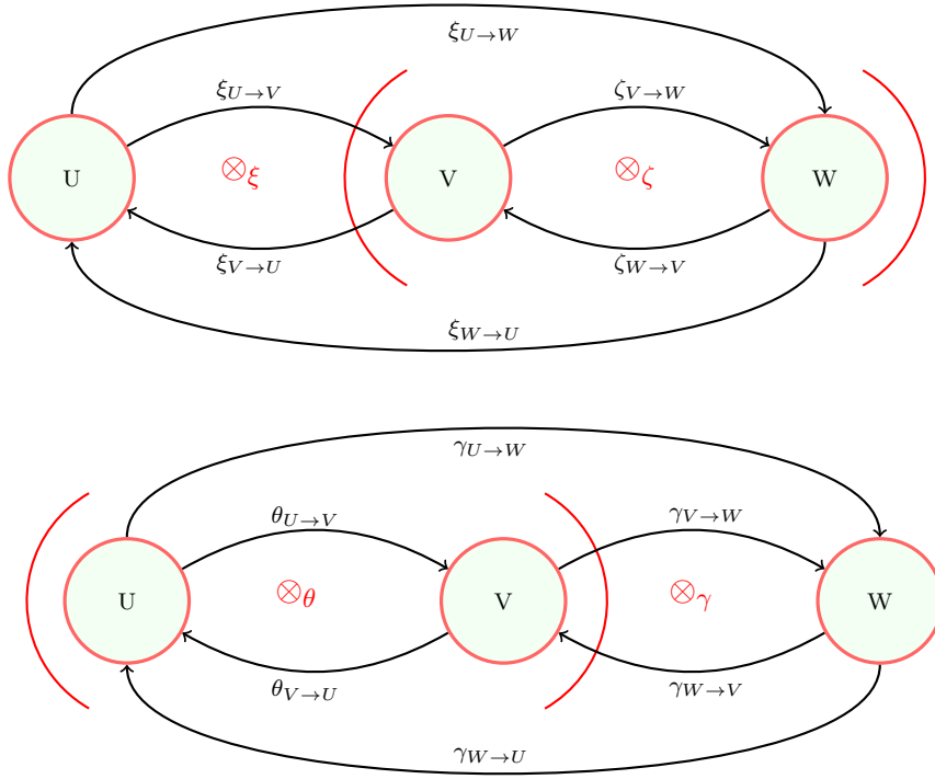
Fig. 2 Proof of associativity
