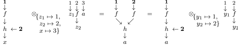
Fig. 7 Another overlap drag
