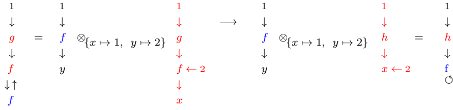
Fig. 4 Rewriting and cycles.
