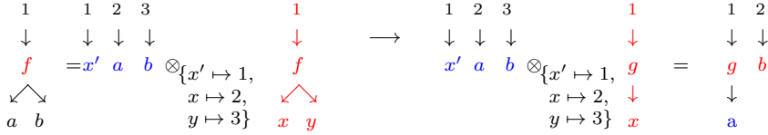
Fig. 5 Rewriting and connected components.
