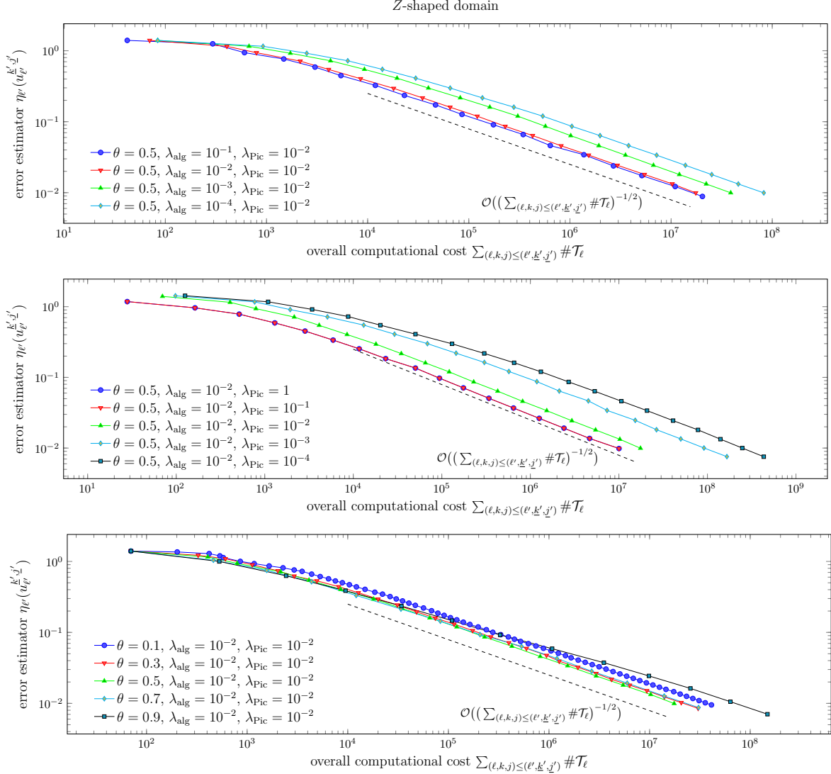
FIGURE 3. Optimal decay rate wrt. overall computational cost, example from Section 7.4. Error estimator \eta_\ell(u_\ell^{k',j'}) on mesh \mathcal{T}_\ell , perturbed Banach–Picard iteration \underline{k}' , and PCG step \underline{j}' of Algorithm 1 with respect to the overall cost expressed as the cumulative sum \sum_{(\ell,k,j) \leq (\ell',k',j')} \#T_\ell for various parameters \theta , \lambda_{\text{Pic}} , and \lambda_{\text{alg}} .
