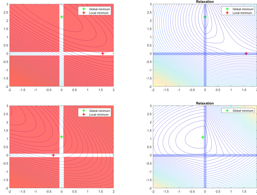
Figure 1: Top: Level lines of the function G_k and G_Q for the example (18). Bottom: Level lines of the function G_k and G_Q for the example (19).
