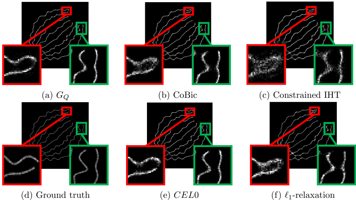
Figure 5: Reconstructed images from the simulated ISBI dataset, 99 non-zero pixels on average. Top: From left to right: G_Q , CoBic and IHT. Bottom: From left to right: Ground Truth, CEL0 , and \ell_1 -relaxation.
