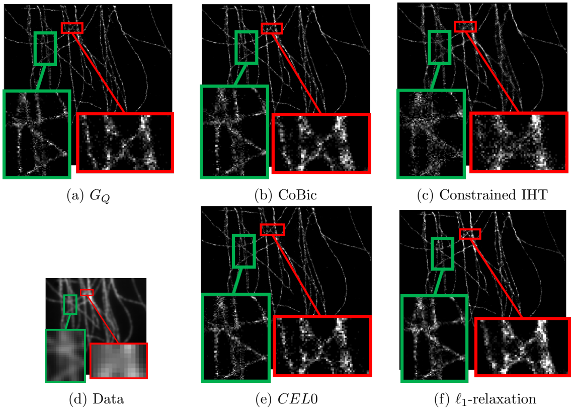
Figure 6: Reconstructed images from the Real ISBI dataset. Top: From left to right: G_Q , CoBic and IHT. Bottom: From left to right: Sum of all acquisitions, CEL0 , and \ell_1 -relaxation.
