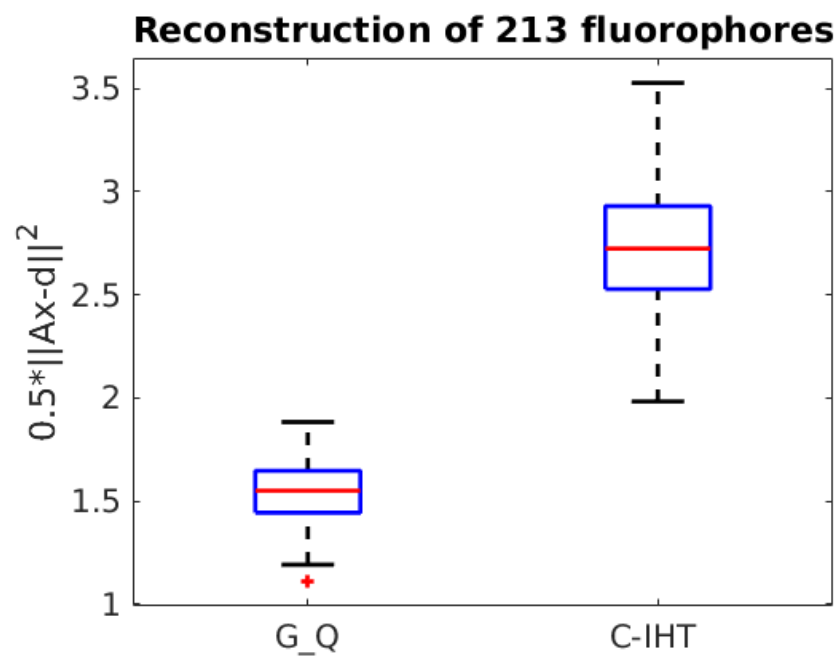
Figure 3: Comparison of the constrained-based algorithms: G_Q and Constrained IHT. The y-axis represent the value \frac{1}{2}\|Ax - d\|^2 . The lower, the better.
