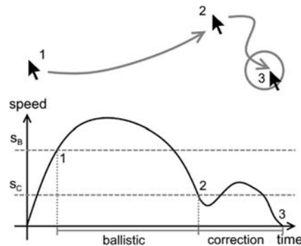
Fig. 1. Target selection example and phase detection. A fast ballistic movement is performed first to roughly bring the cursor close to the desired target (1 -> 2), followed by the slow correction step to exactly select the desired target (2 -> 3).
