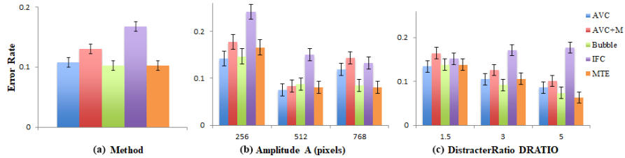
Fig. 8. (a) The mean error rate of different cursor techniques TECHs , and that of grouped by (b) Amplitude A , (c) DistracterRatio DRATIO
