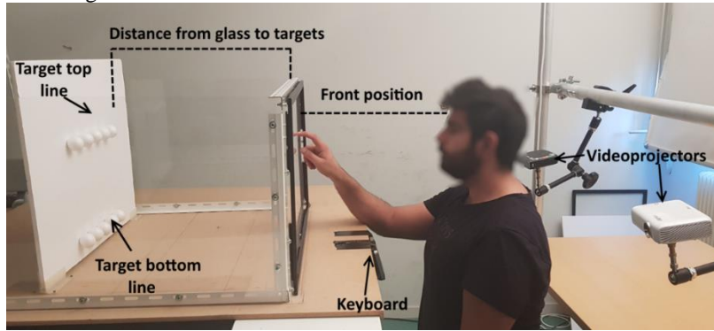
Fig. 5. Experimental setup.
