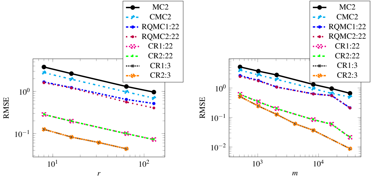
Figure 1: The left panel shows the RMSE for fixed m = 4096 as r increases, and the right panel displays the RMSE for fixed r = 32 as m increases. Both plots have log-log scale. The notation “ d ” in the legend specifies the problem dimension without applying CMC. For CRv:d for d = 3 and 22 , the plots for v = 1 and 2 lie on top of each other.
