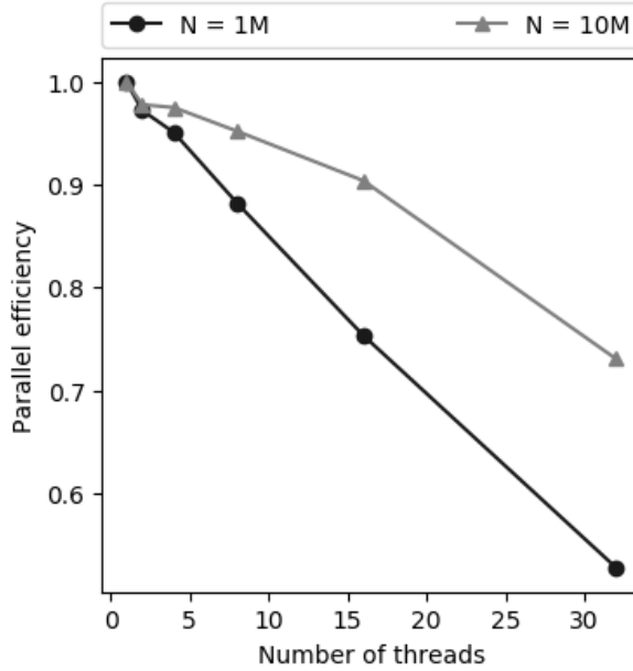
Figure 6: Parallel efficiency for TBFMM using the SPETABARU runtime system and the uniform kernel (order = 8). Test cases: two simulations of one and ten millions of particles randomly distributed in a cube. Hardware: 2 × Intel Xeon Gold 6240 CPU at 2.60GHz with 16 cores each and cache of sizes L1/32K, L2/1024K, L3/25344K.
