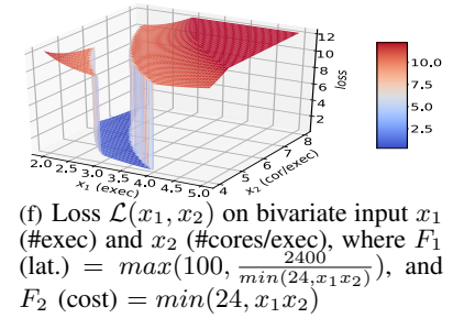
Fig. 3. Constrained optimization with k objectives, and an example \mathcal{C}_{F_1 F_2} “min F_1 (lat.) such that F_1 \in [100, 200] and F_2 (cost) in [8,16] ”
