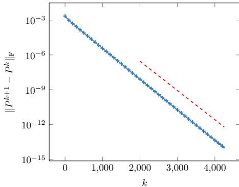
(c) Error decay for SCF and gradient descent algorithms (every few mark only is plotted for the sake of visibility). Marked lines are the evolution of the error \|P^{k+1} - P^k\|_{\text{F}} and dashed lines represents the slope computed with the spectral radius of the Jacobian matrix, computed by finite differences.
