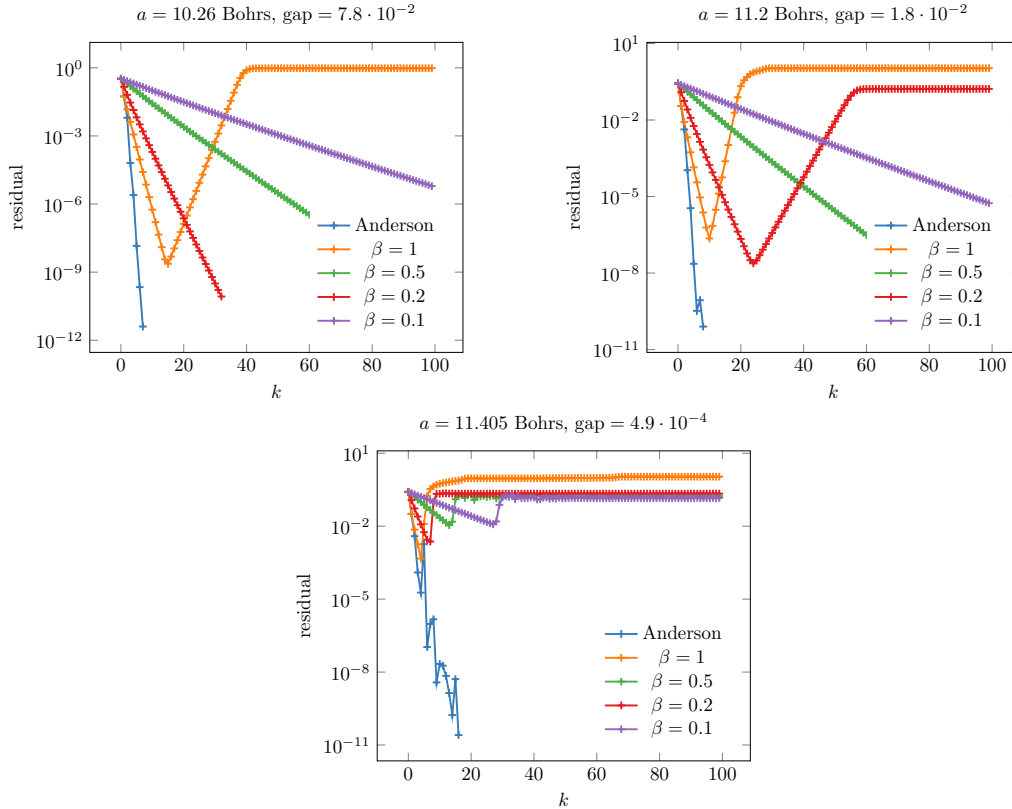
FIGURE 10 – Convergence curves of the density residual as a function of the number of iterations k for Silicon with different lattice constants a .
