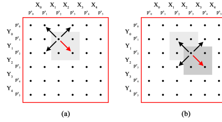
Fig. 7. (a) If depth change was detected at point (p_2^x, p_1^y) , then scan through (p_1^x, p_0^y) , (p_3^x, p_0^y) , (p_1^x, p_2^y) , (p_3^x, p_2^y) , as indicated by the black arrows. Another detection of depth change was found at (p_3^x, p_2^y) , as indicated by the red arrow, thus it is selected as a block placement at layer 1. (b) If there is another depth change at (p_3^x, p_2^y) , we conduct the same diagonal-point-scanning process to detect the block at (X_3, Y_2) at layer 2.
