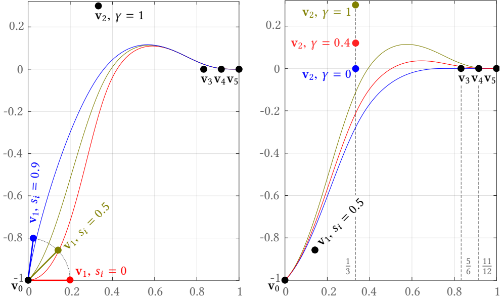
Fig. 5. Profile curves. The control points v_0 and v_5 are fixed to ensure surface continuity. The position of v_1 is constrained to the circular arc with center (0, -1) and radius 0.2 and fully determined by the slope angle \theta_i at the evaluation vertex i (left). The ordinate of v_2 is optimized according to the user-defined bulging parameter \gamma (right). The abscissas of v_2 , v_3 and v_4 can be edited for additional artistic control of the bulge position and shape.
