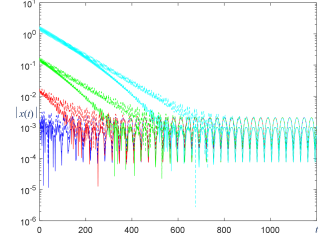
Fig. 3. Trajectories with \alpha = 0.9 and d \neq 0
