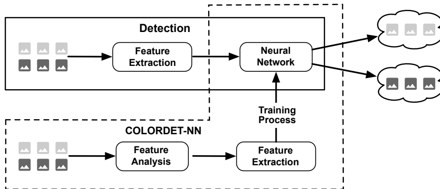
Figure 1. ColorDet-NN approach.
