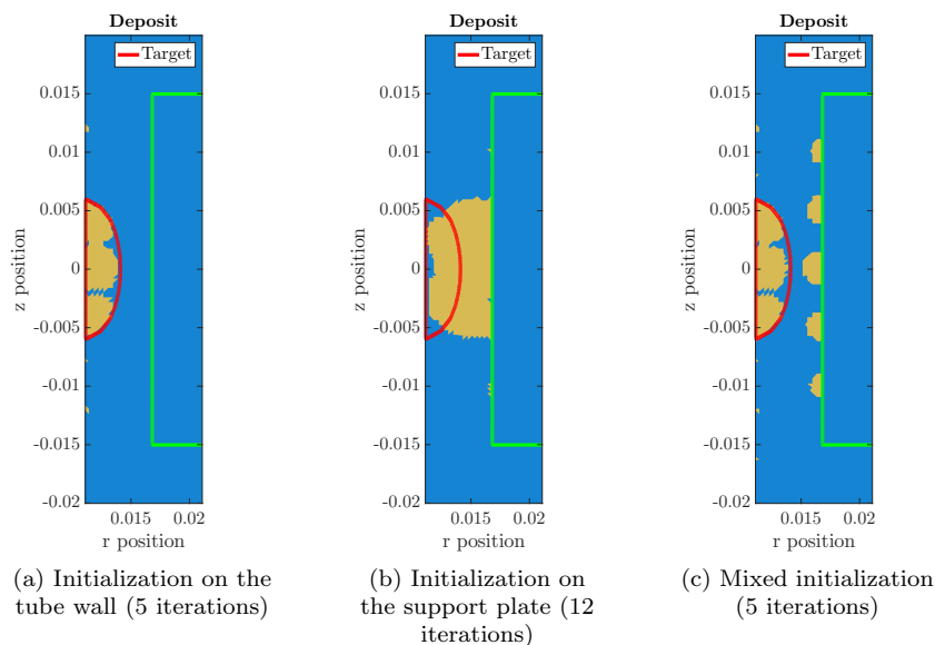
Figure 4.0.13: Optimal shape (in yellow) computed by the reconstruction algorithm for different initializations. In red, the shape to reconstruct.
