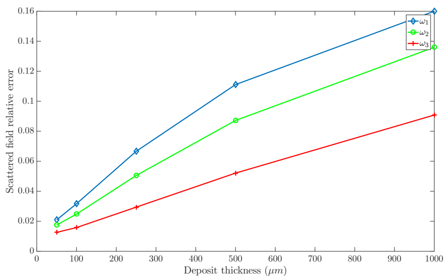
Figure 4.0.20: Relative error for the scattered field, for each pulsation
