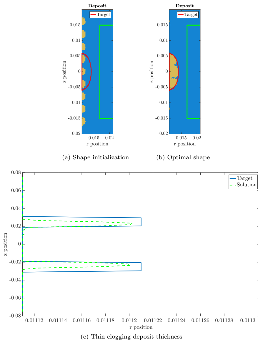
Figure 4.0.24: Optimal solution (12 iterations) for a shape optimization problem with thin clogging deposits
