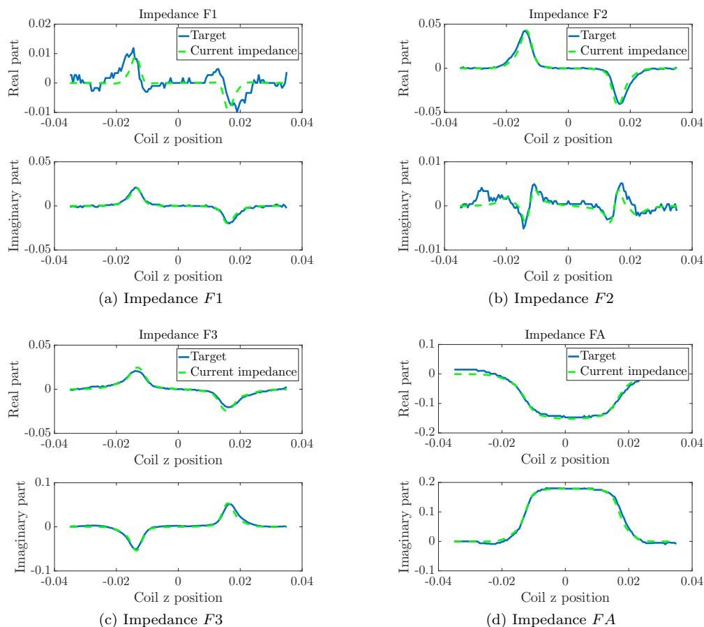
Figure 4.0.33: Data fitting for the impedance signals for the optimal \mu and \sigma .
