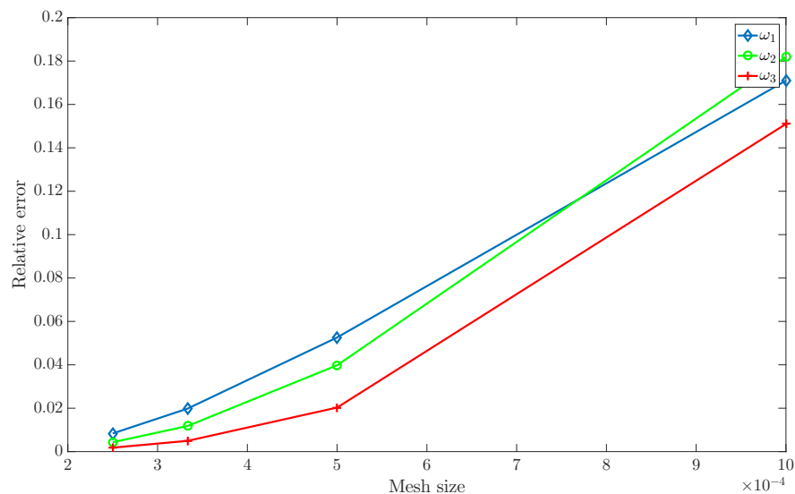
Figure 4.0.10: Relative error for the scattered field, for each pulsation
