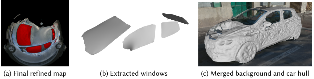
Fig. 6. At the end of the MRF step we obtain the final window mask (a, in red, drawn over the reprojected texture). This map is used to separate the window meshes (b) from the merged background/interior and car hull meshes (c).
