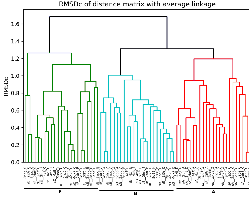
Figure 3: Clustering the AcrB asymmetric monomers restricted to subdomains (Loop2, Loop8, Loop11, TM, \alpha -helix) (section 3.2) with RMSD Comb yields three clusters corresponding to the A/B/E states. Green: cluster E, Cyan: cluster B, Red: cluster A.
