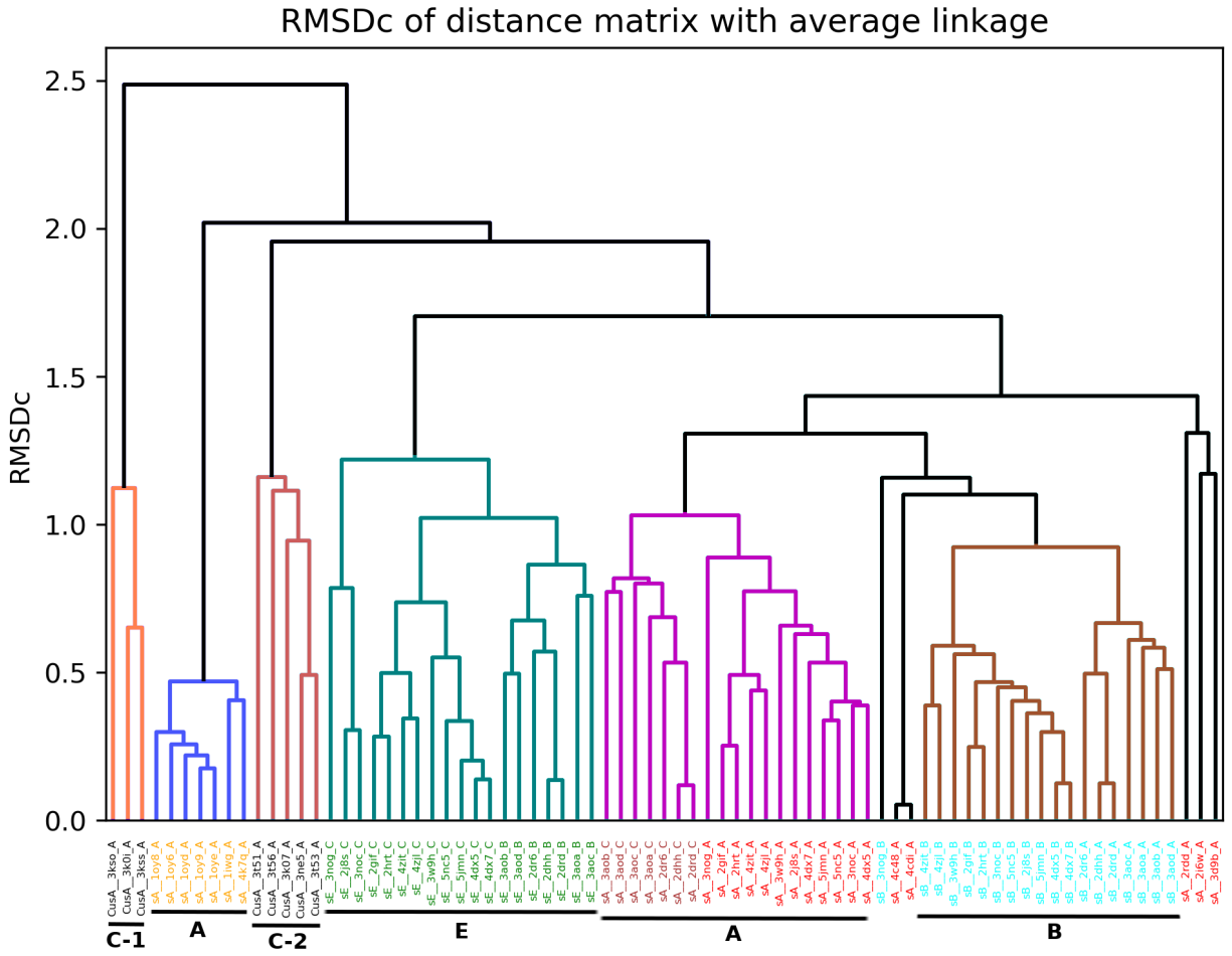
Figure 14: RMSD Comb between AcrB and CusA . RMSD was computed on selected subdomains (Loop2, Loop11, TM). See Section 4.4.1
