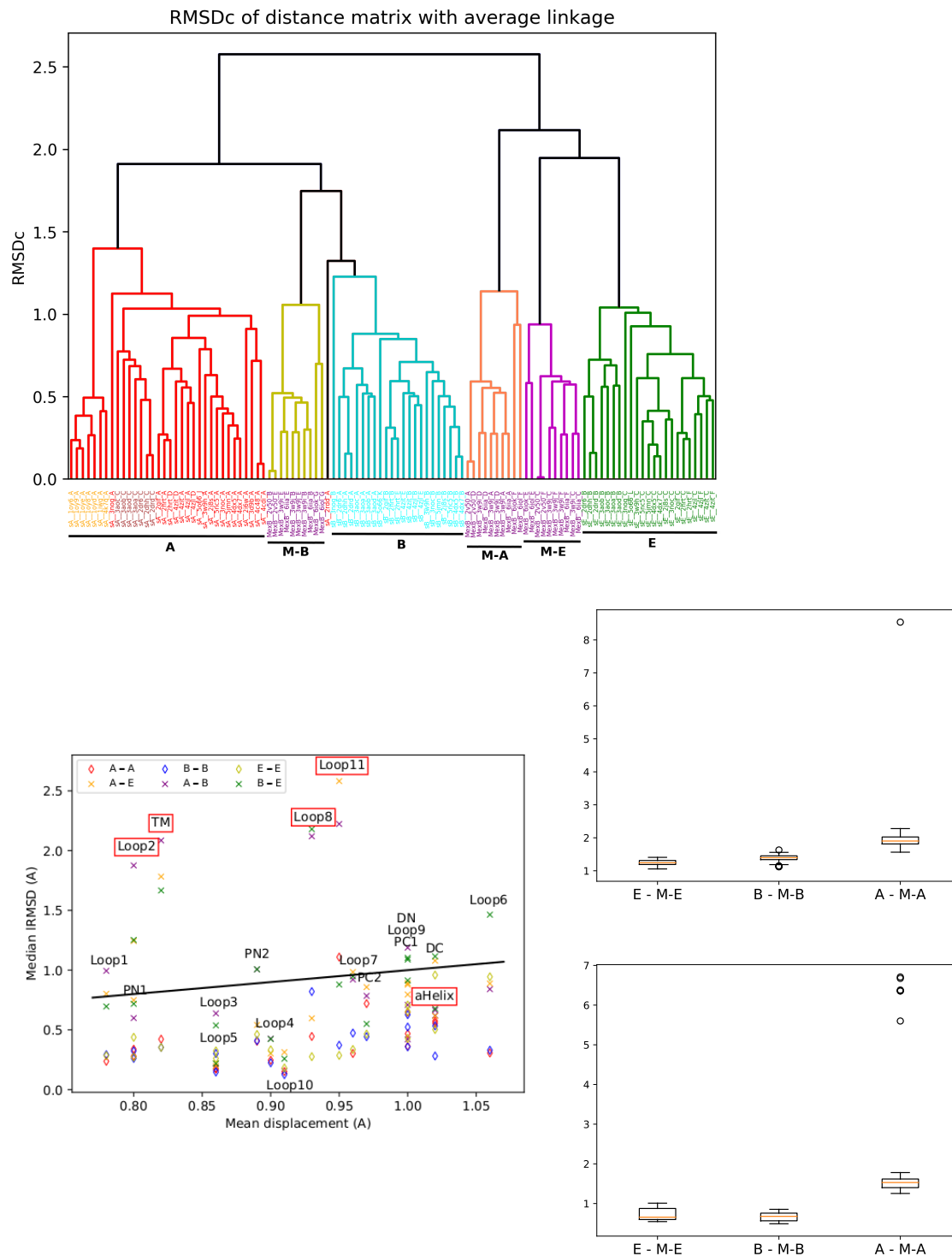
Figure 6: Analysis of MexB's states. (First row) Clustering with RMSD_{Comb} for AcrB and MexB. RMSD was computed on domains (TM, porter, funnel ) (Second row, left) Characterization of dynamic subdomains of MexB. Mean square displacement in crystal asymmetric structures versus median IRMSD. (Second row, right) States of AcrB versus states of MexB. On a per state basis, boxplot of IRMSD values (Å) for pairs of domains from AcrB and MexB. Top: Porter Domain; bottom: TM Domain.
