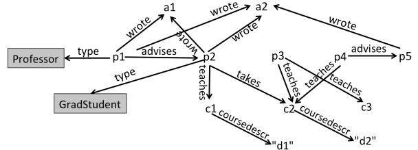
FIGURE 2. Sample RDF graph.
