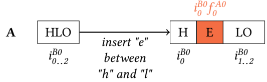
Figure 2. Insertion leading to longer identifiers
