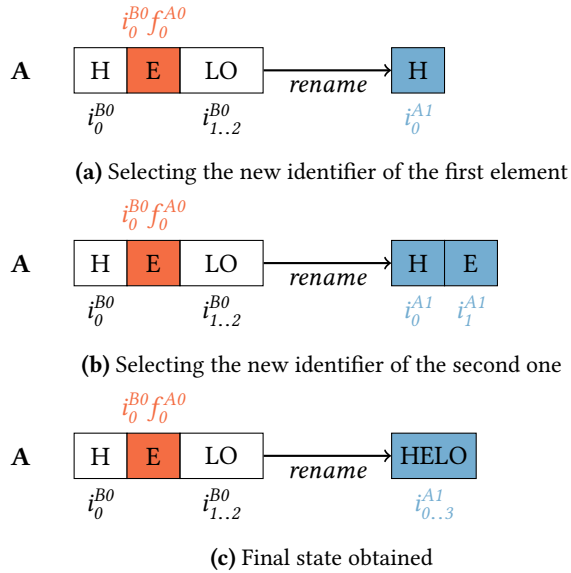
Figure 3. Renaming the sequence
