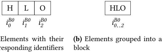
Figure 1. Representation of a LogootSplit sequence containing the elements "HLO"
