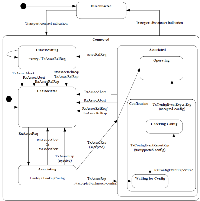
Fig. 3. State machine of the IEEE 11073 PHD Manager
