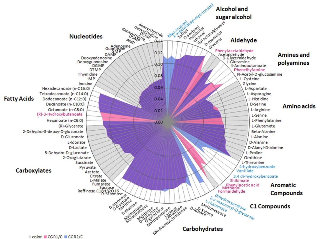
Figure 5. In silico analyses of potential substrates used by Microbacterium sp CGR1 and CGR2. The circle graph shows the predicted maximum growth rates (in 1/h) for each substrate shown. Color key: Pink for CGR1, blue for CGR2 and purple for both strains. Color key for substrate names indicates presence of such substrate in the model: pink for CGR1, blue for CGR2 and black for both. Note that presence does not imply carbon/energy source, as it is in the case of phenylalanine. Grey and white background are intended to separate substrates by families as follows: Grey for: aldehydes, amino acids, carboxylates and nucleotides; white for alcohol and sugar alcohol, amines and polyamines, aromatic compounds, carbohydrates, and fatty acids.
