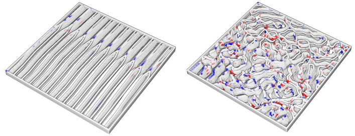
Fig. 19. Two slabs of tool paths visualized in our printer emulation tool. A red color indicates an overhang violation, a blue color an overlap. Sliced with 0.2 mm layers for a 0.4 mm nozzle, cube filled at 25% density. Left: \Gamma = 0 . Right: \Gamma = \frac{\pi}{2} .
