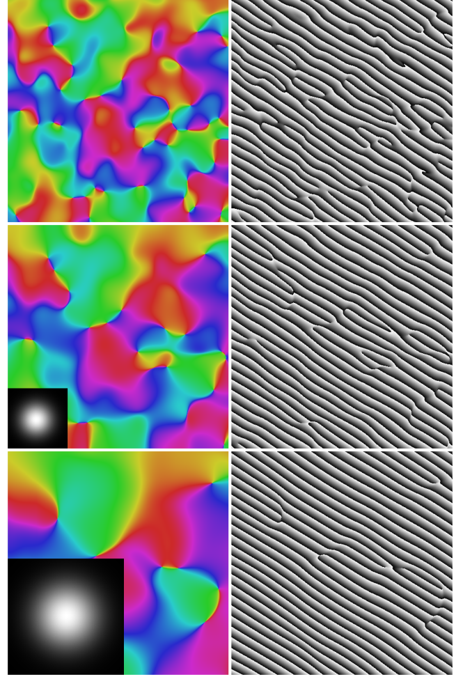
Fig. 10. Phasor noise filtering with increasing filter kernel sizes. Left : phasor field argument, encoded as hue. Right : phasor sawtooth. Inset : filtering kernel. Top to bottom : increasing kernel size. Note how the phasor field becomes smoother and remaining singularities become point singularities.
