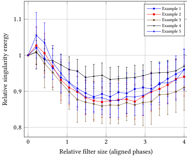
Fig. 17. Relative change of singularity energy as the filter size increases. The filter radius is defined relative to the noise kernel radius. All points are computed with 20 phase alignment iterations. As in Figure 16, results are averaged over 50 samples to reduce noise. The energy reduction reaches a minimum value at a relative filter size of 2 (the filter bandwidth is 1/\sqrt{2} the noise kernel bandwidth) on all examples. When the filter size increases beyond the tipping point, we tend toward a unique phase shift per direction of oscillation. Such a global choice of phase is not valid for a varying direction field, reducing the filter performance. The relative reduction in energy is weaker than what the regularization achieves (at best 15% on these examples) as illustrated by Figure 15, however this still improves the visual result significantly.
