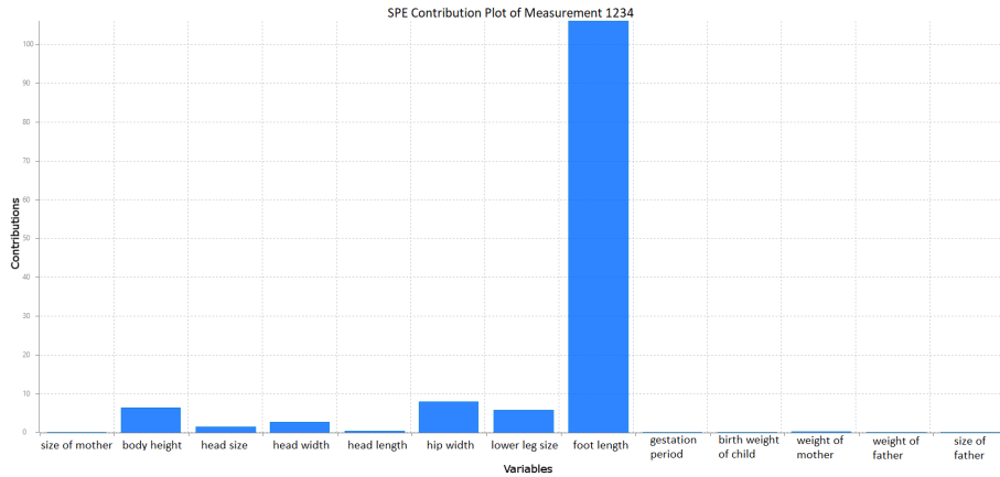
Fig. 4. A squared prediction error contribution plot example of the red marked measurement in Figure 3 on the first principal component. As shown by the figure, the foot length contributes the most to this record. When going back to the raw data, this record shows a rather high value in the variable foot length compared to the other observations.
