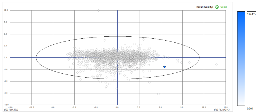
Fig. 10. The score plot (based on the second PCA result computed in Section 3.2) of the first and the second principal component, characterizing the x-axis and y-axis. The color scheme represents the SPE-values of each record. Small deviations (between the actual and the predicted model) are colored white, whereas high differences are highlighted in darker color.
