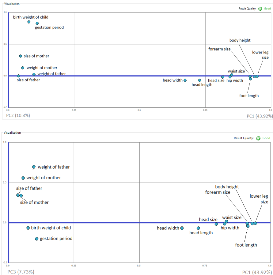
Fig. 9. Loadings plots based on the second PCA result computed in Section 3.2. The first graph illustrates the loadings plot of the first and the second principal component, characterizing the x-axis and y-axis. On the second graph, the x-axis and the y-axis depict the first and the third principal component. The location of the PCA-transformed variables plotted on the graph provides insight into the strength of correlation between the original variables and the influence of a variable on the specific component.
