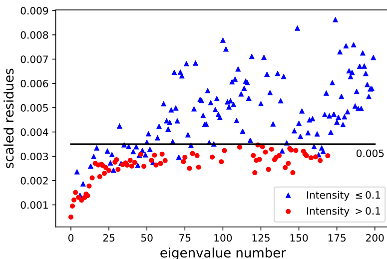
FIG. 10. Scaled residues using the SI strategy ( \varepsilon_I = 0.1\text{ km/mol} ). Calculations are done for C_2H_4O with the following parameters: F = 200 , p = 4 , \varepsilon = 3.5 \times 10^{-3} and E_{max} = 20000\text{ cm}^{-1} .
