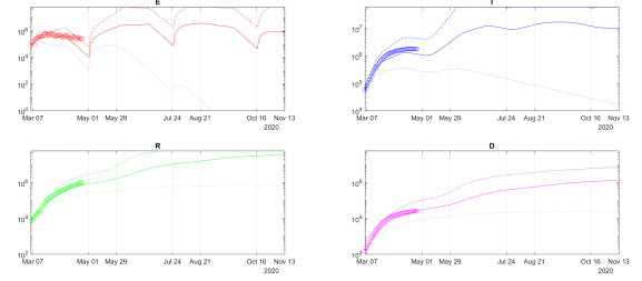
Fig. 9. The results of simulation of (5) for Italy under \pm 10\% variation of all parameters
