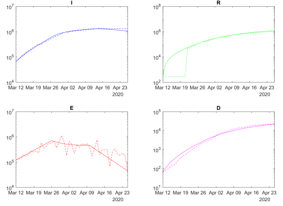
Fig. 5. The results of verification with identified parameters
