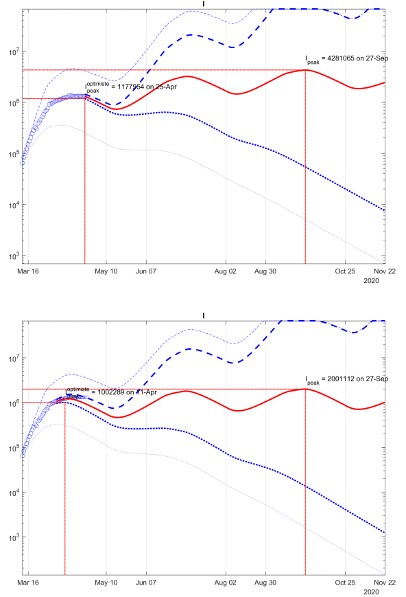
Fig. 7. Validation of prediction of I for France with J and J - 20 points of data under deviations of values of all parameters
