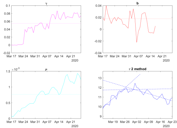
Fig. 14. The identified parameters for Germany
