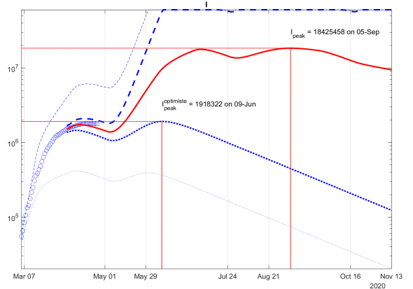
Fig. 10. Validation of prediction of I for Italy with J and J - 20 points of data under deviations of values of all parameters
