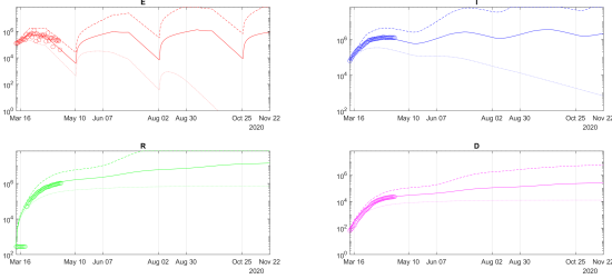
Fig. 6. The results of simulation of (5) for France under \pm 10\% variation of all parameters
