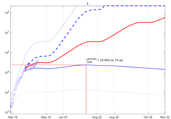
Fig. 19. Validation of prediction of I for Brazil with J and J - 20 points of data under deviations of values of all parameters
