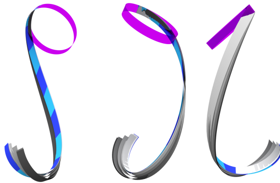
Figure 7: Comparison of our method (in blue) with the FENICS-SHELL finite element code implementing the Naghdi shell model (six increasing width/thickness ratios depicted with different gray levels), under three different viewpoints (see accompanying video).
