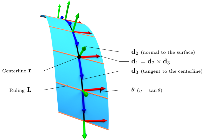
Figure 2: Base parameterization of a ribbon consisting of the centerline \mathbf{r} , the Cosserat material frame \mathcal{R} , and the scalar field \eta = \tan \theta .
