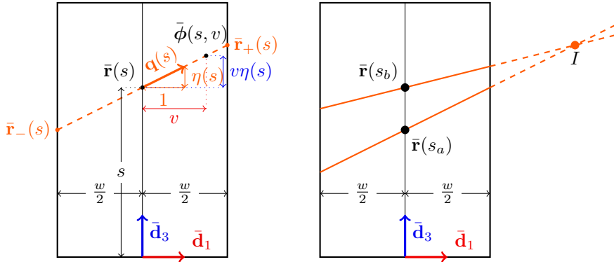
Figure 3: On the left, parameterization of the ribbon with s , v and \eta , on the flattened configuration. On the right, illustration of a singular point. Rulings passing at the points of arc lengths s_a and s_b are drawn in orange. The surface of the ribbon being developable and smooth, rulings are not allowed to intersect inside the ribbon.
