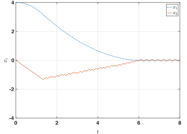
Fig. 4. System states for explicit scheme x_{i+1} = x_i + hF(x_i)
