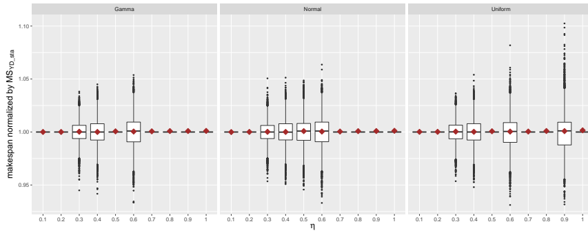
Figure 20: Boxplots represent the performance of the optimal static strategy for k_{static} . Brown diamonds plot optimal theoretical makespan M_{the\_sta}^{OPT} .
