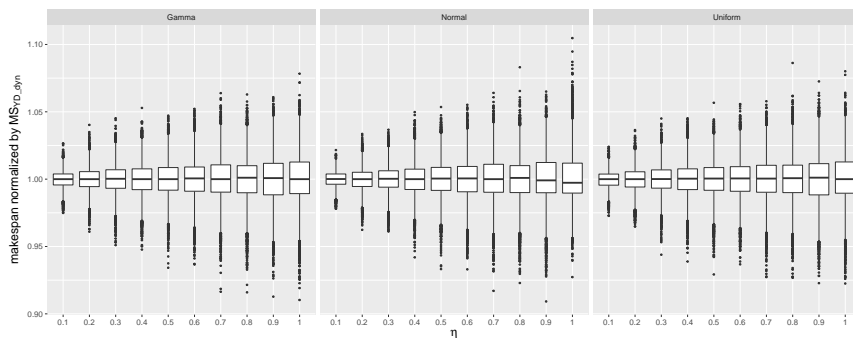
Figure 22: Boxplots represent the performance of the optimal dynamic strategy for W_{th} .
