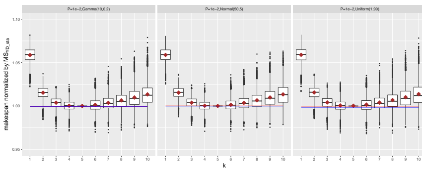
Figure 14: Boxplots represent the performance of the static strategy that chooses k . Brown diamonds plot \mathbb{E}[MS_{\mathcal{D}}](k) (theoretical makespan). The blue (resp. red) line represent the makespan obtained by the optimal dynamic strategy \overline{MS}_{sim\_dyn}(W_{th}) (resp. the YD-dynamic strategy \overline{MS}_{YD\_dyn} ).
