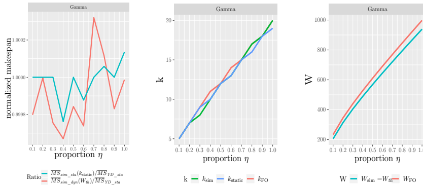
Figure 5: Simulation with varying the proportion of checkpoint time \eta to the expected iteration time.
