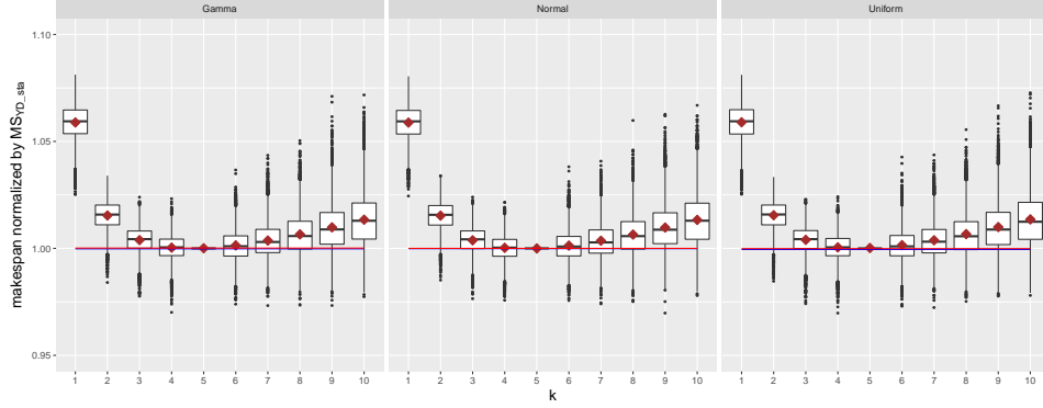
Figure 1: Boxplots represent the performance of the static strategy that chooses k . Brown diamonds plot \mathbb{E}[MS_{\mathcal{D}}](k) (theoretical makespan). The blue (resp. red) line represents the makespan obtained by the optimal dynamic strategy \overline{MS}_{sim\_dyn}(W_{th}) (resp. the YD-dynamic strategy \overline{MS}_{YD\_dyn} ).
