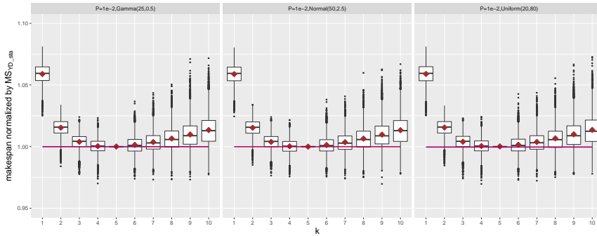
Figure 7: Boxplots represent the performance of the static strategy that chooses k . Brown diamonds plot \mathbb{E}[MS_{\mathcal{D}}](k) (theoretical makespan). The blue (resp. red) line represent the makespan obtained by the optimal dynamic strategy \overline{MS}_{sim\_dyn}(W_{th}) (resp. the YD-dynamic strategy \overline{MS}_{YD\_dyn} ).
