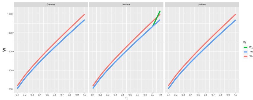
Figure 21: W of static strategy simulation with varying proportion \eta .
