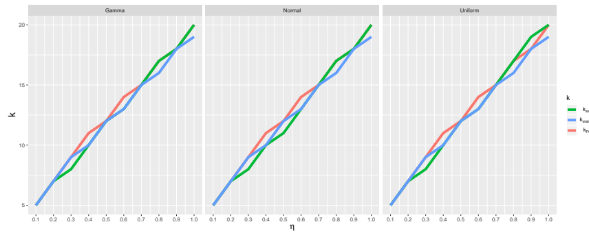
Figure 19: k of static strategy simulation with varying proportion \eta .
