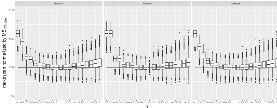
Figure 2: Boxplots represent the performance of the dynamic strategy that chooses a threshold of \gamma \cdot W_{\text{th}} . The orange (resp. purple) line represents the makespan obtained by the optimal static strategy \overline{MS}_{\text{sim\_sta}}(k_{\text{static}}) (resp. the YD-static strategy \overline{MS}_{\text{YD\_sta}} ).
