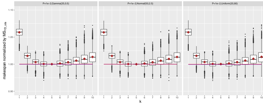
Figure 13: Boxplots represent the performance of the static strategy that chooses k . Brown diamonds plot \mathbb{E}[MS_{\mathcal{D}}](k) (theoretical makespan). The blue (resp. red) line represent the makespan obtained by the optimal dynamic strategy \overline{MS}_{sim\_dyn}(W_{th}) (resp. the YD-dynamic strategy \overline{MS}_{YD\_dyn} ).
