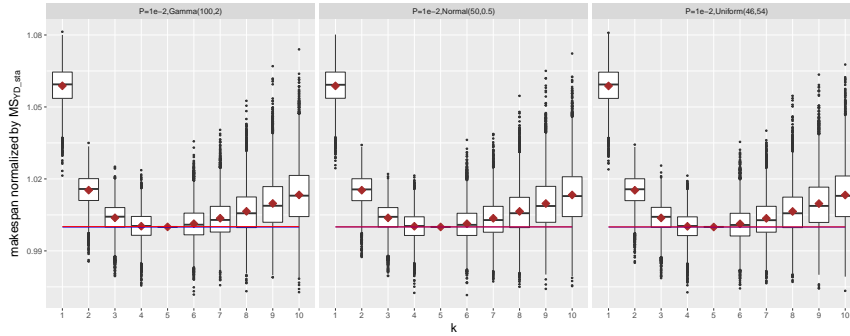
Figure 12: Boxplots represent the performance of the static strategy that chooses k . Brown diamonds plot \mathbb{E}[MS_{\mathcal{D}}](k) (theoretical makespan). The blue (resp. red) line represent the makespan obtained by the optimal dynamic strategy \overline{MS}_{sim\_dyn}(W_{th}) (resp. the YD-dynamic strategy \overline{MS}_{YD\_dyn} ).
