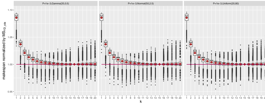
Figure 6: Boxplots represent the performance of the static strategy that chooses k . Brown diamonds plot \mathbb{E}[MS_{\mathcal{D}}](k) (theoretical makespan). The blue (resp. red) line represent the makespan obtained by the optimal dynamic strategy \overline{MS}_{sim\_dyn}(W_{th}) (resp. the YD-dynamic strategy \overline{MS}_{YD\_dyn} ).
