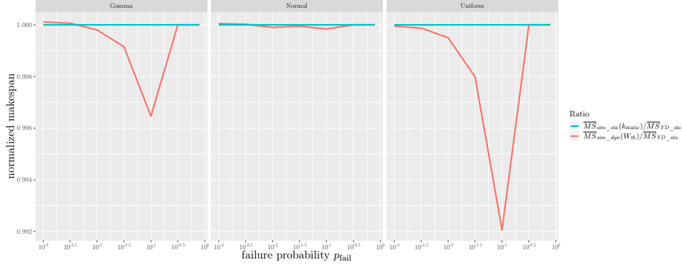
Figure 3: Simulation with varying failure probability
