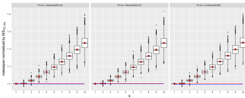
Figure 8: Boxplots represent the performance of the static strategy that chooses k . Brown diamonds plot \mathbb{E}[MS_{\mathcal{D}}](k) (theoretical makespan). The blue (resp. red) line represent the makespan obtained by the optimal dynamic strategy \overline{MS}_{sim\_dyn}(W_{th}) (resp. the YD-dynamic strategy \overline{MS}_{YD\_dyn} ).
