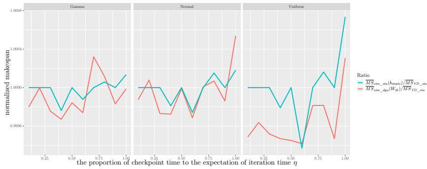
Figure 18: Simulation with varying the proportion of checkpoint time to the expectation of iteration time
