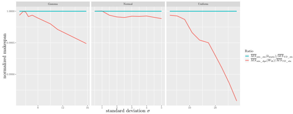
Figure 4: Simulation with varying standard deviation
