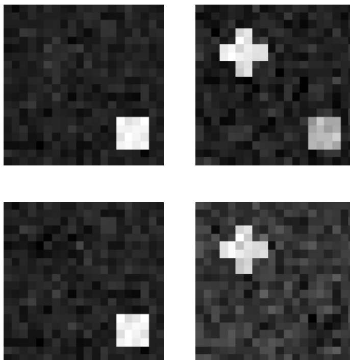
Figure S15. Estimated sources by EM (up) and tmp-EM (down). The two real sources were correctly identified by tmp-EM, but EM did not fully separate the cross and the square.
