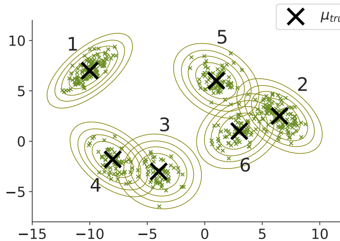
Figure S1. 500 sample points from a Mixture of Gaussians with 6 classes. The true centroid of each Gaussian are depicted by black crosses, and their true covariance matrices are represented by the confidence ellipses of level 0.8, 0.99 and 0.999 around the centre.
