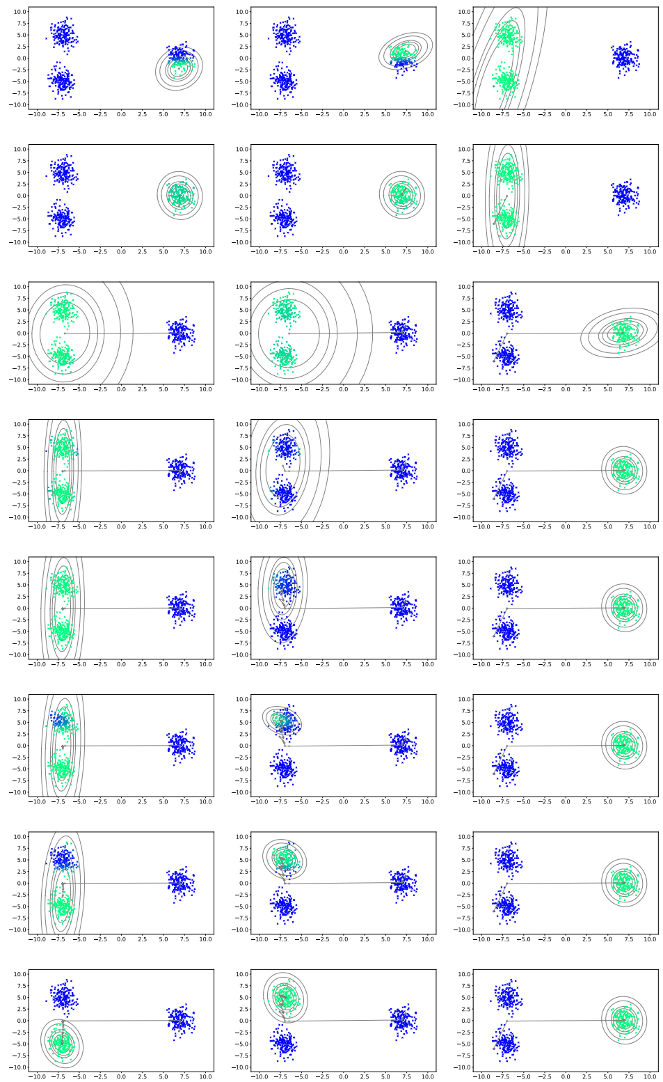
Figure S10. Paths of the centroids for tmp-EM with the "2v1" initialization. Parameter set 1 (least ambiguous).
