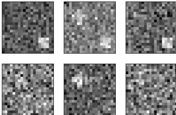
Figure S14. 6 typical observation obtained with the source mixing model. With the noise, the sources are harder to identify.
