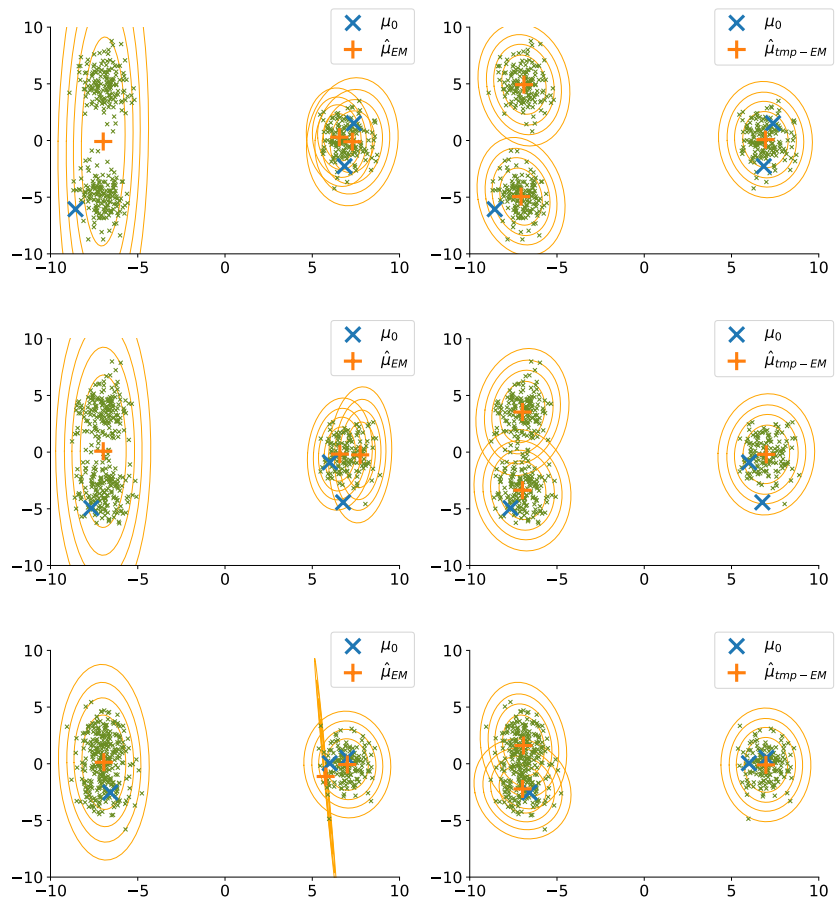
Figure S8. Typical final positioning of the centroids by EM (left column) and tmp-EM (right column) when the initialisation is made by selecting two points in the isolated cluster and one in the lower ambiguous cluster (blue crosses). The three rows represent the three gradually more ambiguous parameter sets. Each figure represents the positions of the estimated centroids after convergence of the EM algorithms (orange cross), with their estimated covariance matrices (orange confidence ellipses). In each simulation, 500 sample points were drawn from the real GMM (small green crosses). In those examples, although EM kept two centroids on the isolated cluster, tmp-EM managed to correctly identify the position of the three real centroids.
