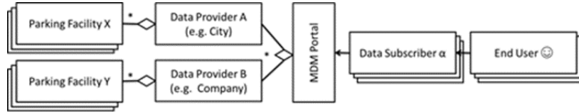
Fig. 1. A Data flow of parking information through the MDM portal ( Legend: ◇ Aggregation)
